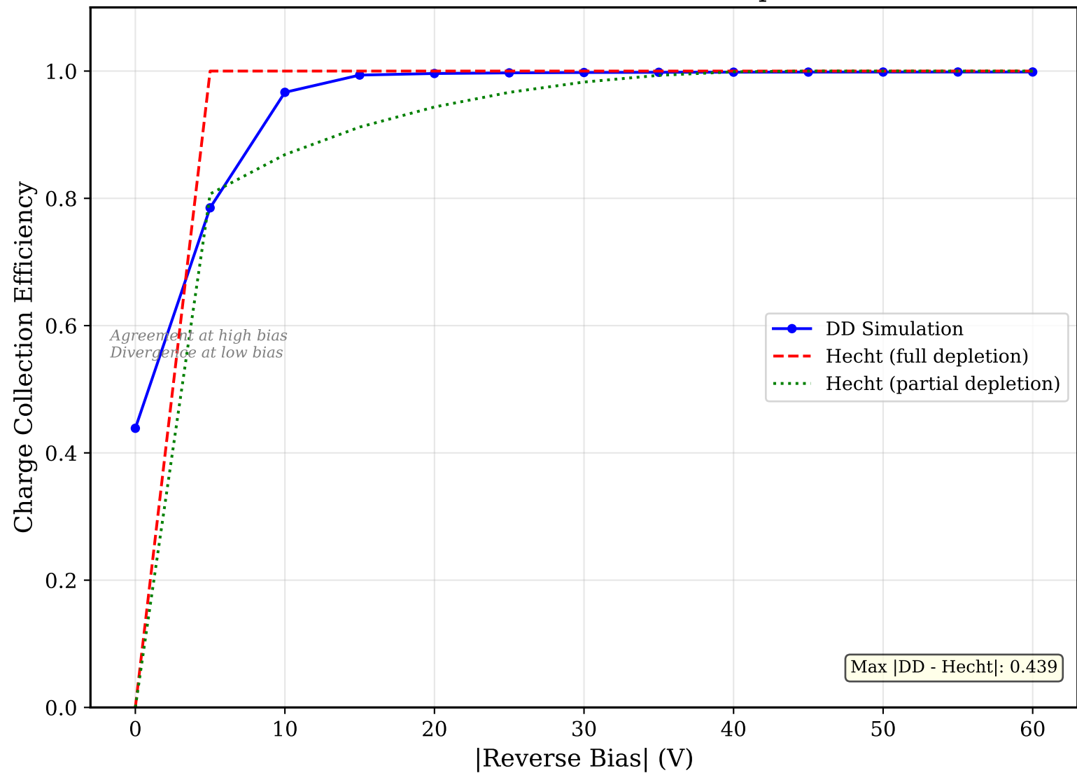
CCE: DD Simulation vs Hecht Equation
