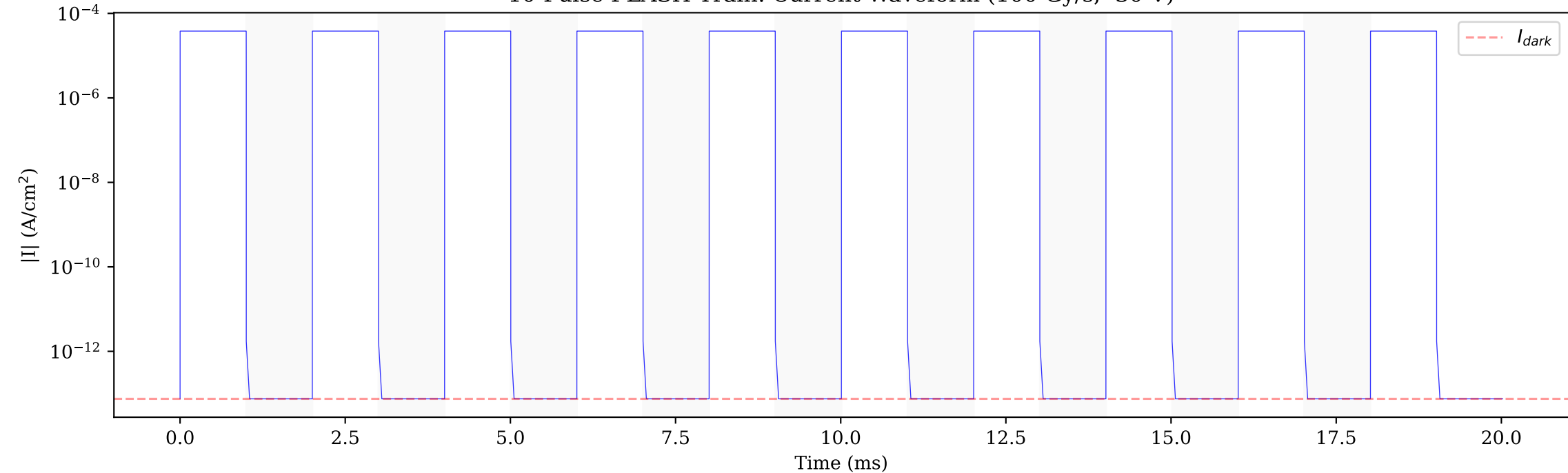
10-Pulse FLASH Train: Current Waveform (100 Gy/s, -30 V)
