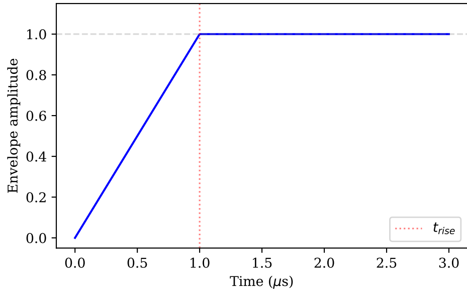
Rise transient ( t_{rise} = 1 \mu s )
