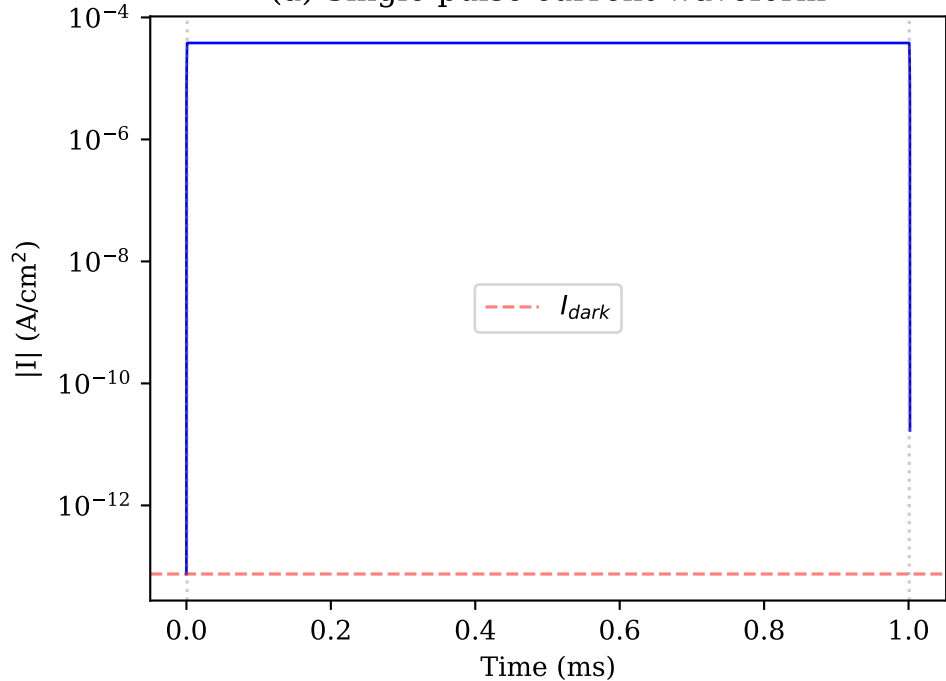
(a) Single-pulse current waveform
