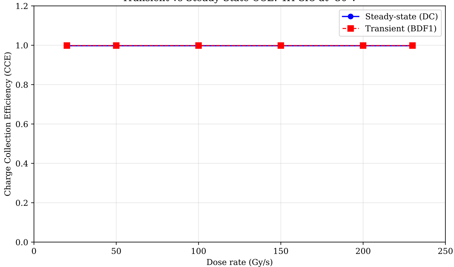
Transient vs Steady-State CCE: 4H-SiC at -30 V
