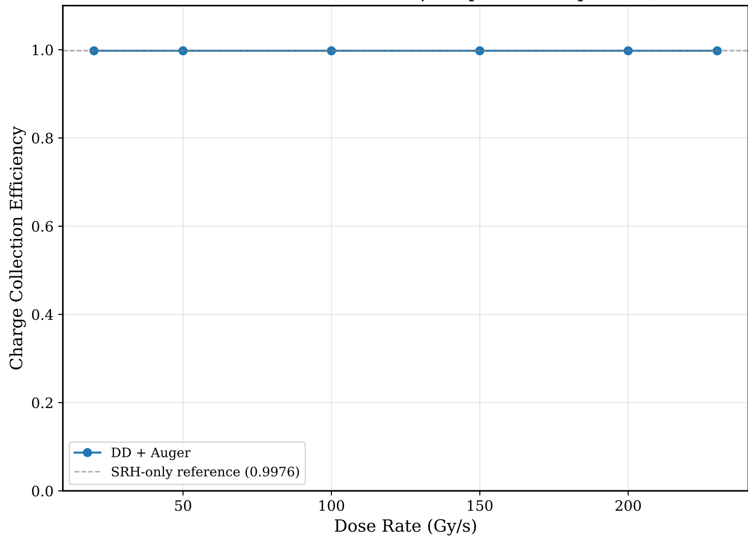
CCE vs Dose Rate (-30V, 10 \mu\text{m} epi, 62 MeV protons)
