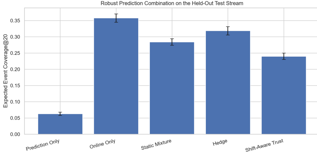
Figure 3: Final robust-learning comparison on the held-out sequential test stream. Error bars show 95% normal-approximation intervals over user-level mean losses.
