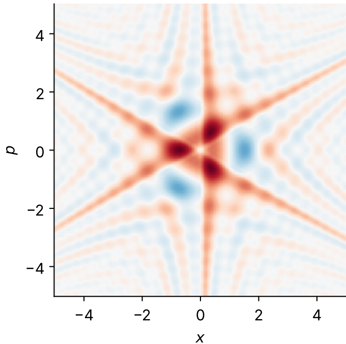
|S_3\rangle : P_3 = 0.707 vs classical 0.667
