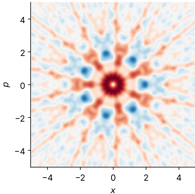
|S_7\rangle : P_7 = 0.607 vs classical 0.571
