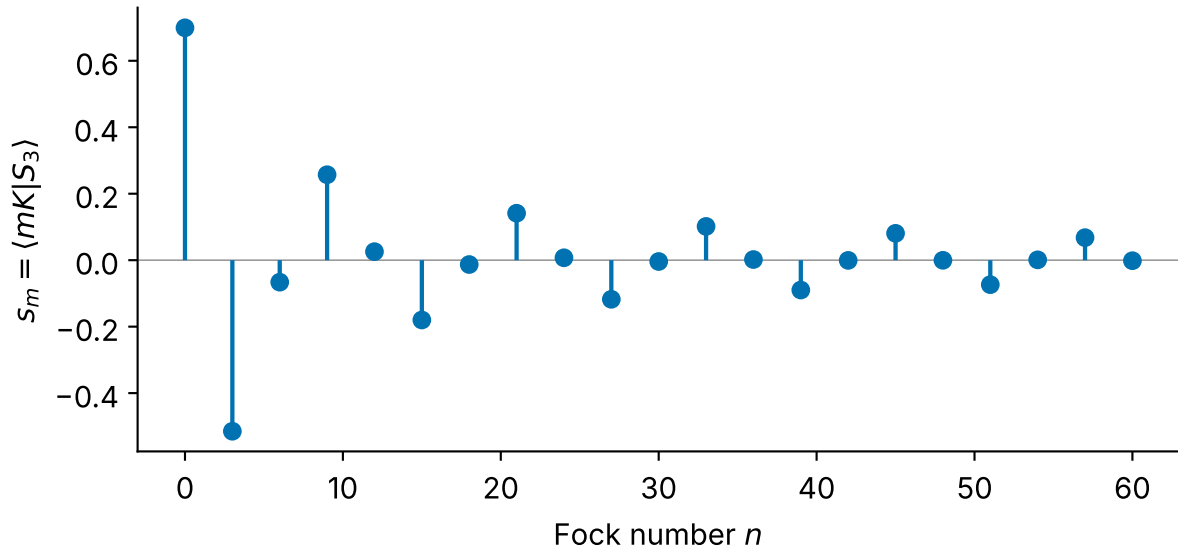
Fock-grid coefficients of the spider state |S_3\rangle
