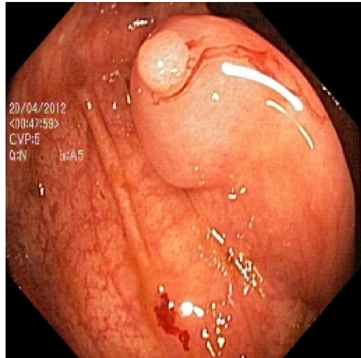
Input Image
