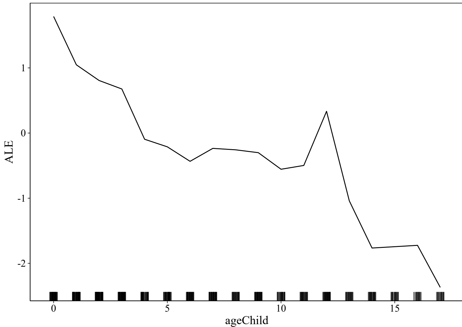
ALE plot: ageChild
