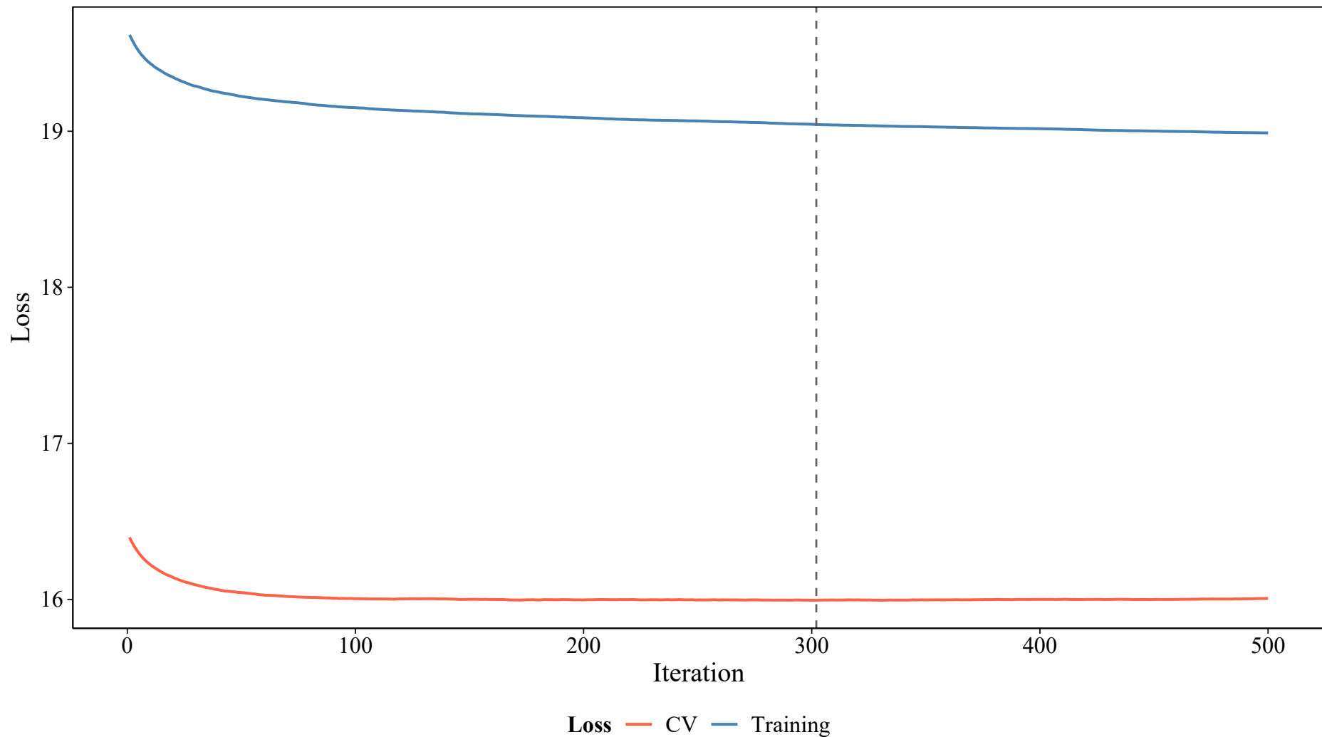
GBM: training vs. CV loss
