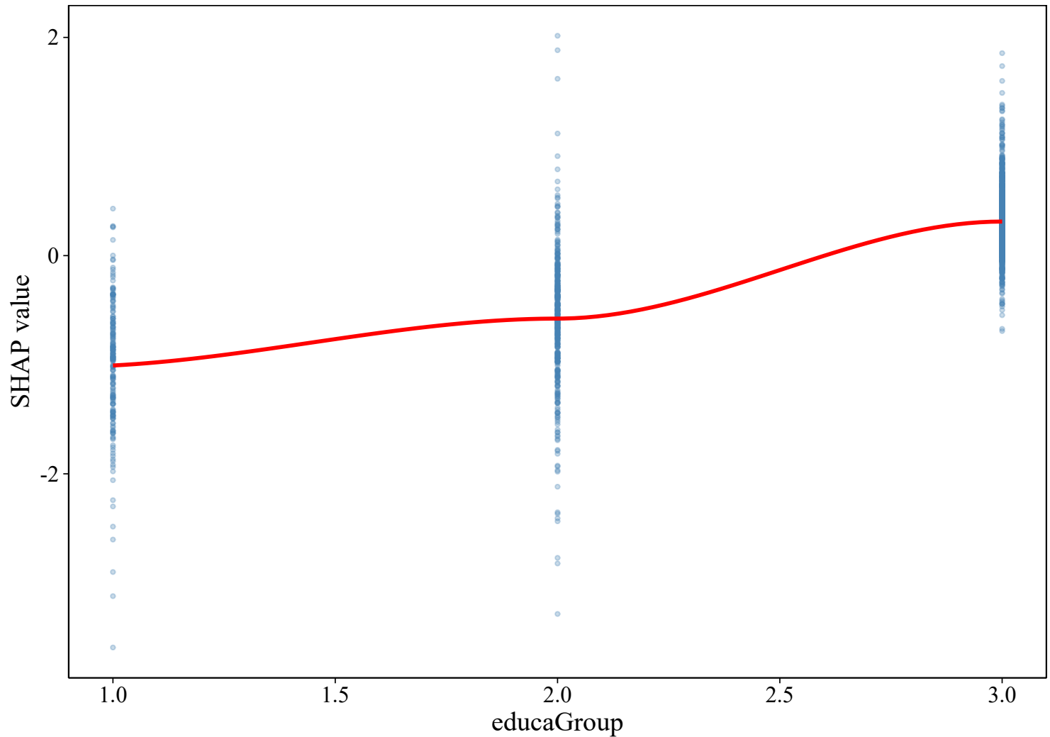
SHAP: educaGroup
