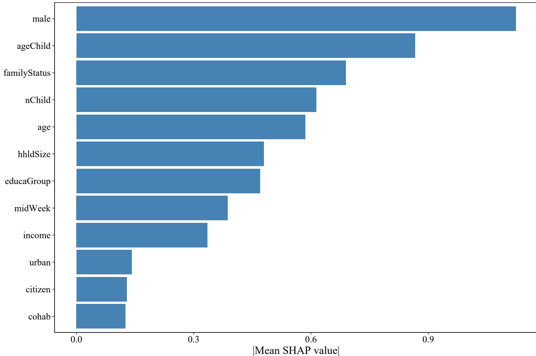
SHAP Feature Importance (RSF)
