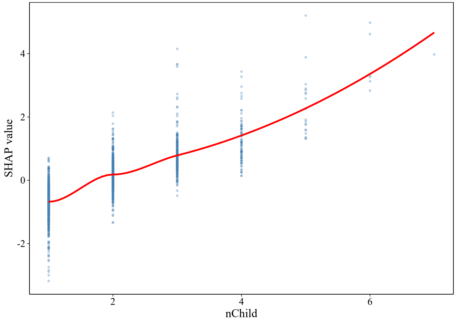
SHAP: nChild
