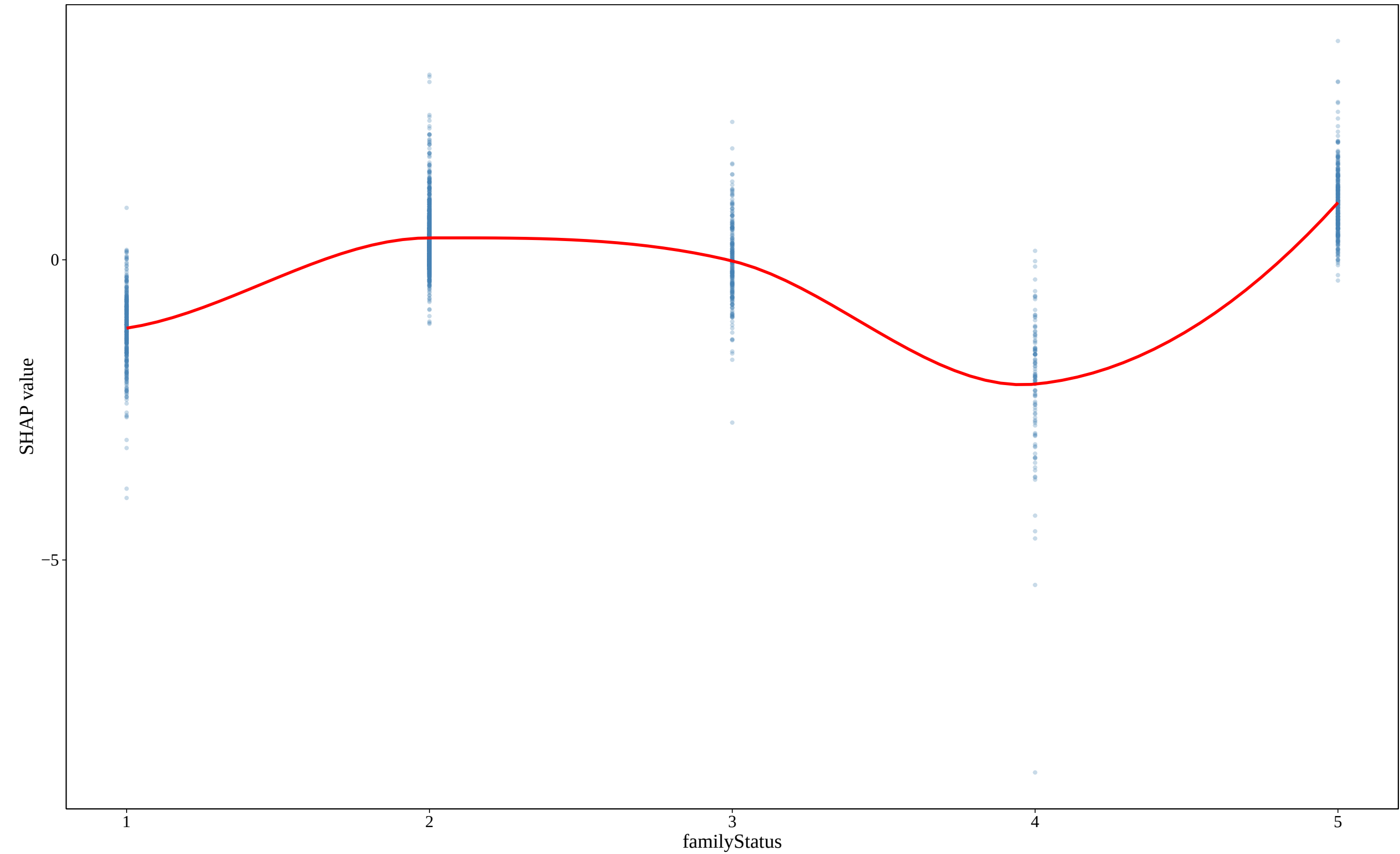
SHAP: familyStatus
