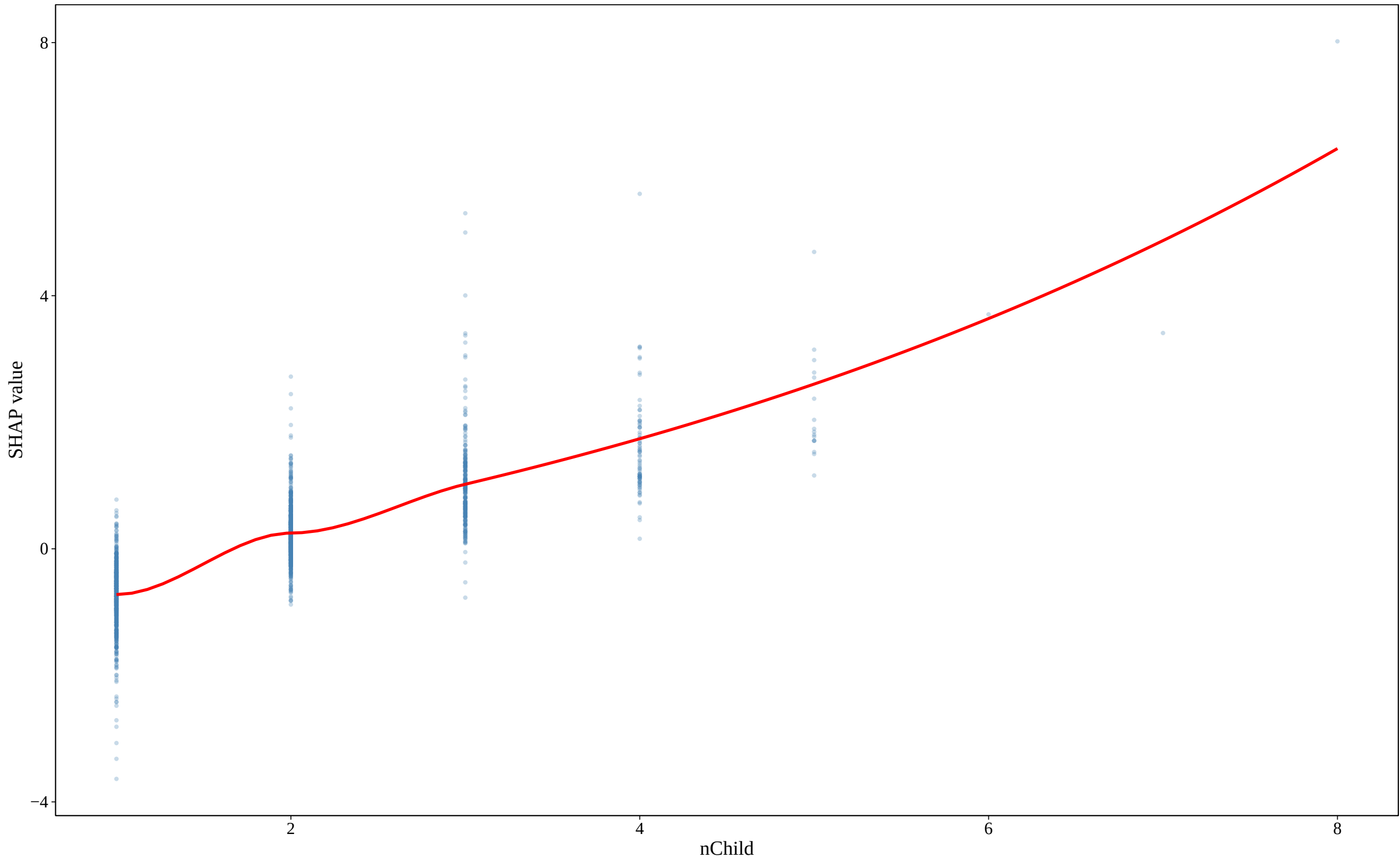
SHAP: nChild
