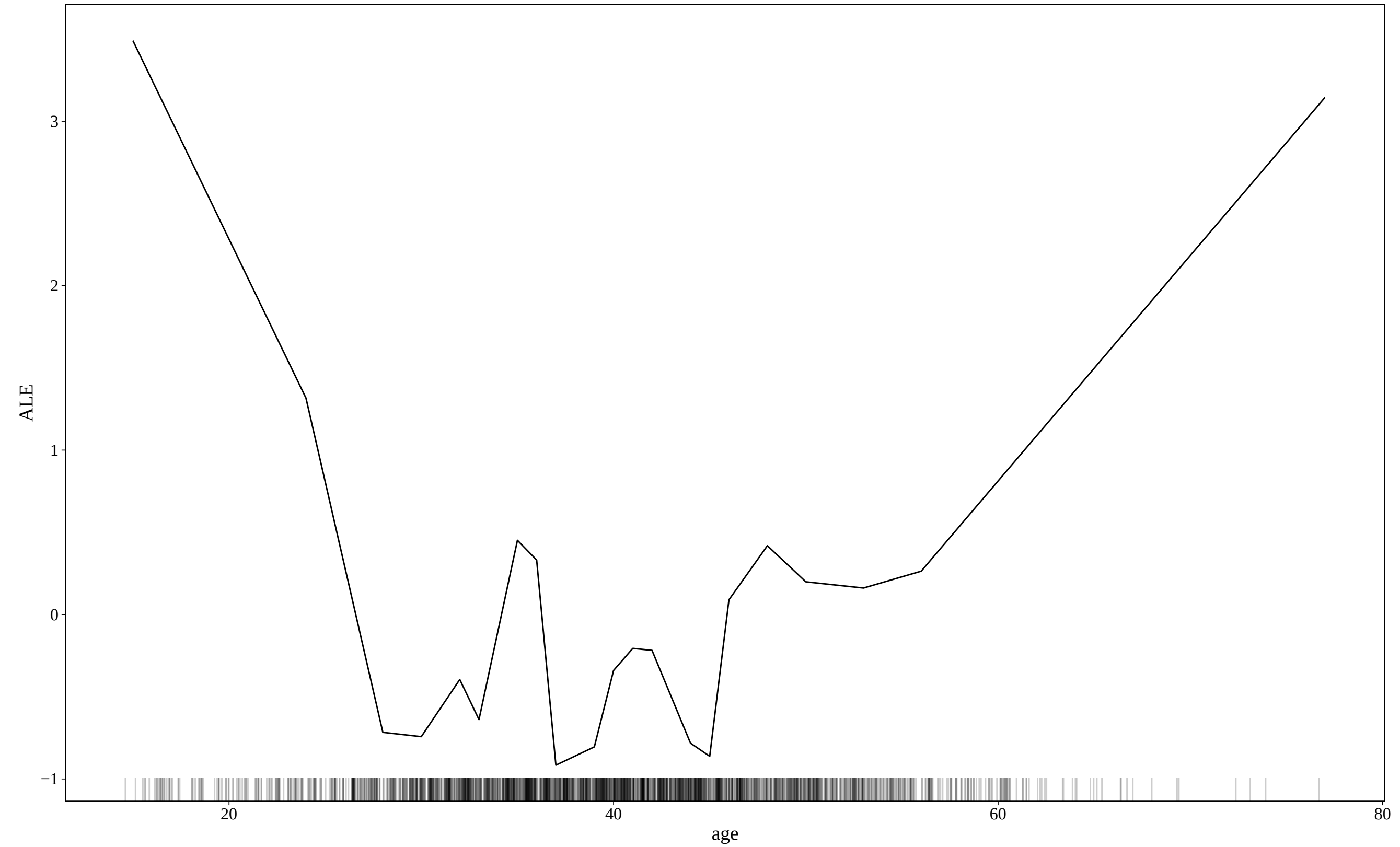
ALE plot: age
