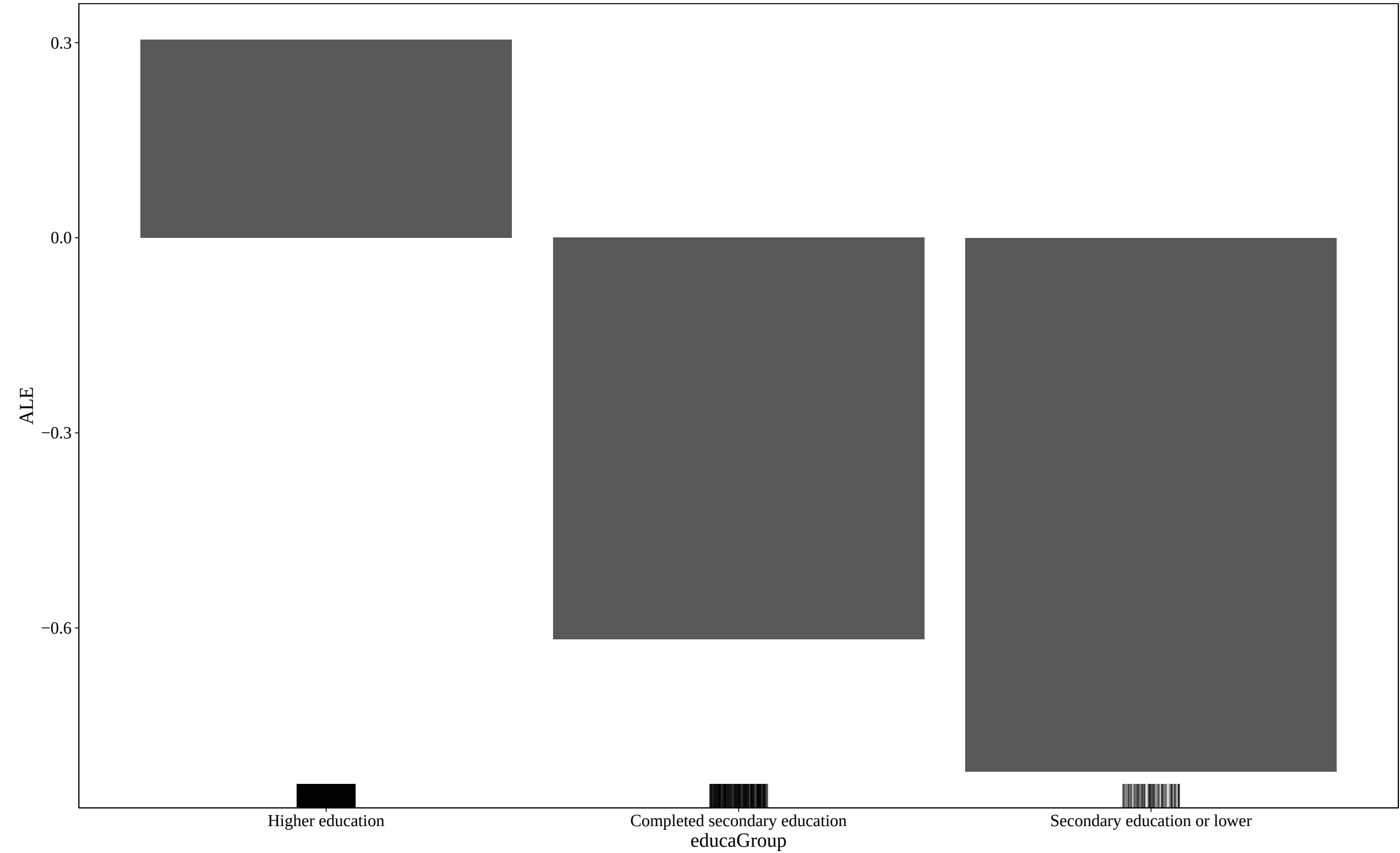
ALE plot: educaGroup
