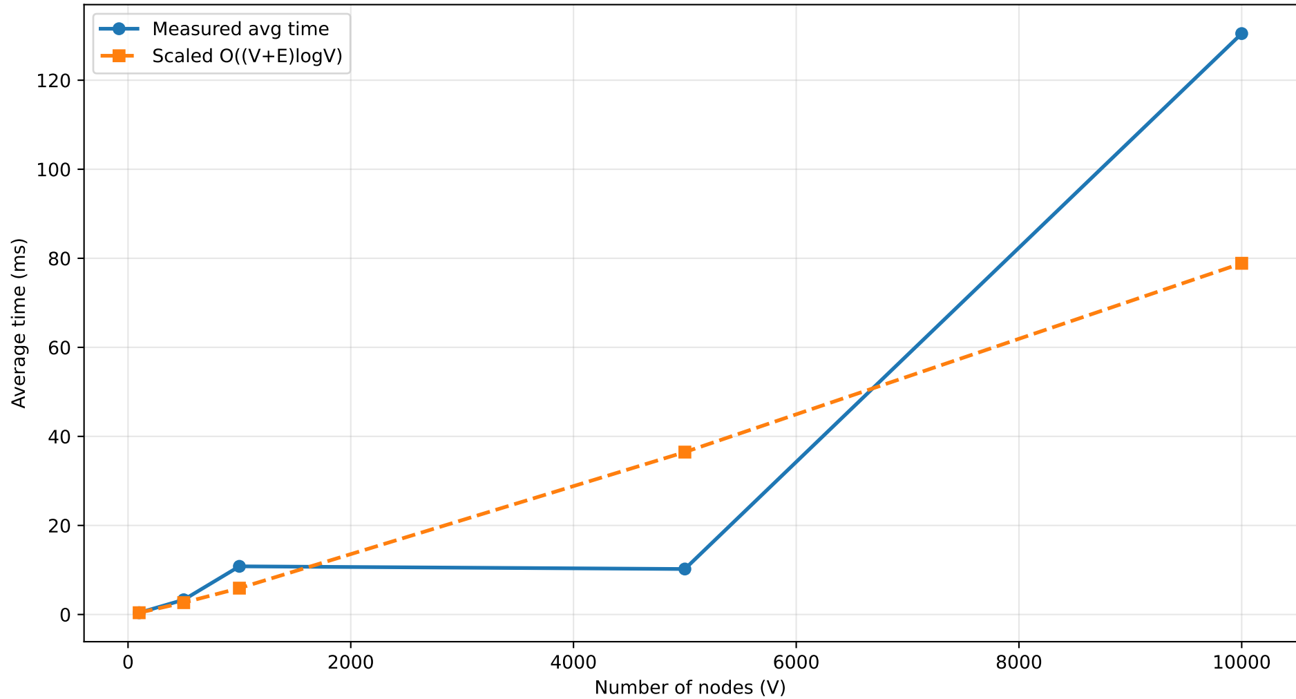
Dijkstra Performance Test
