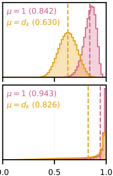
Diagonal KDN
