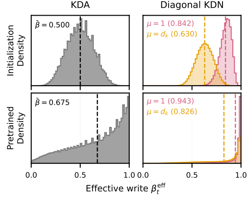
Figure 2: Effective-write distributions before (top) and after 50B-token pretraining (bottom). Diagonal KDN overlays \mu = 1 and \mu = d_k ; dashed lines mark pooled means.
