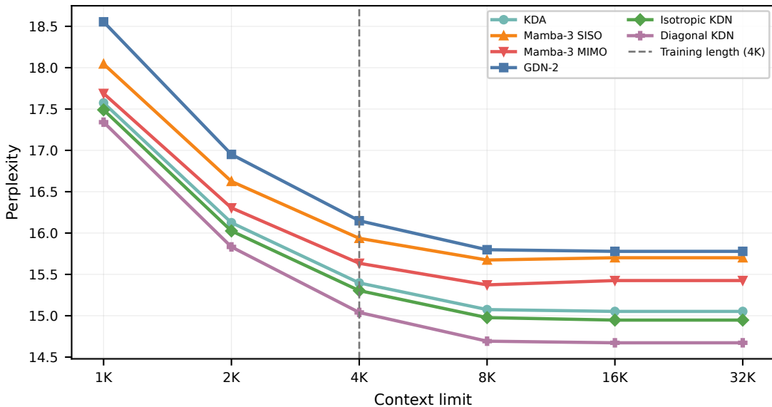
WikiText word PPL — Recurrent 1.3B models
