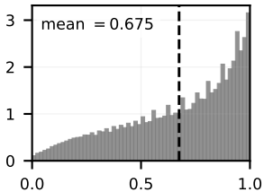
After pretraining Density
