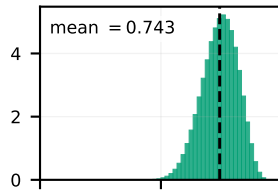
Diagonal KDN \mu = \sqrt{d_k}
