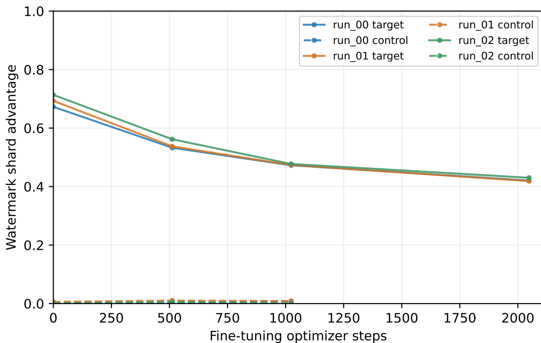
Continuous clean fine-tuning: 600,000 distinct examples, 1 epoch — 15/42 audits complete
