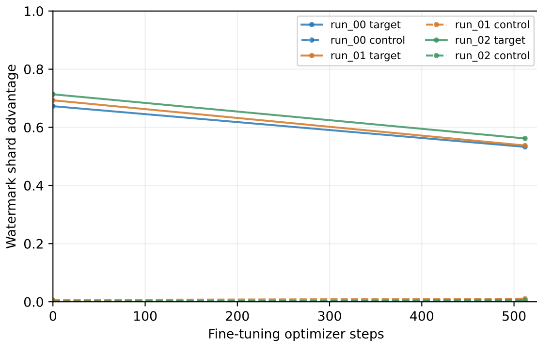
Continuous clean fine-tuning: 600,000 distinct examples, 1 epoch — 6/42 audits complete
