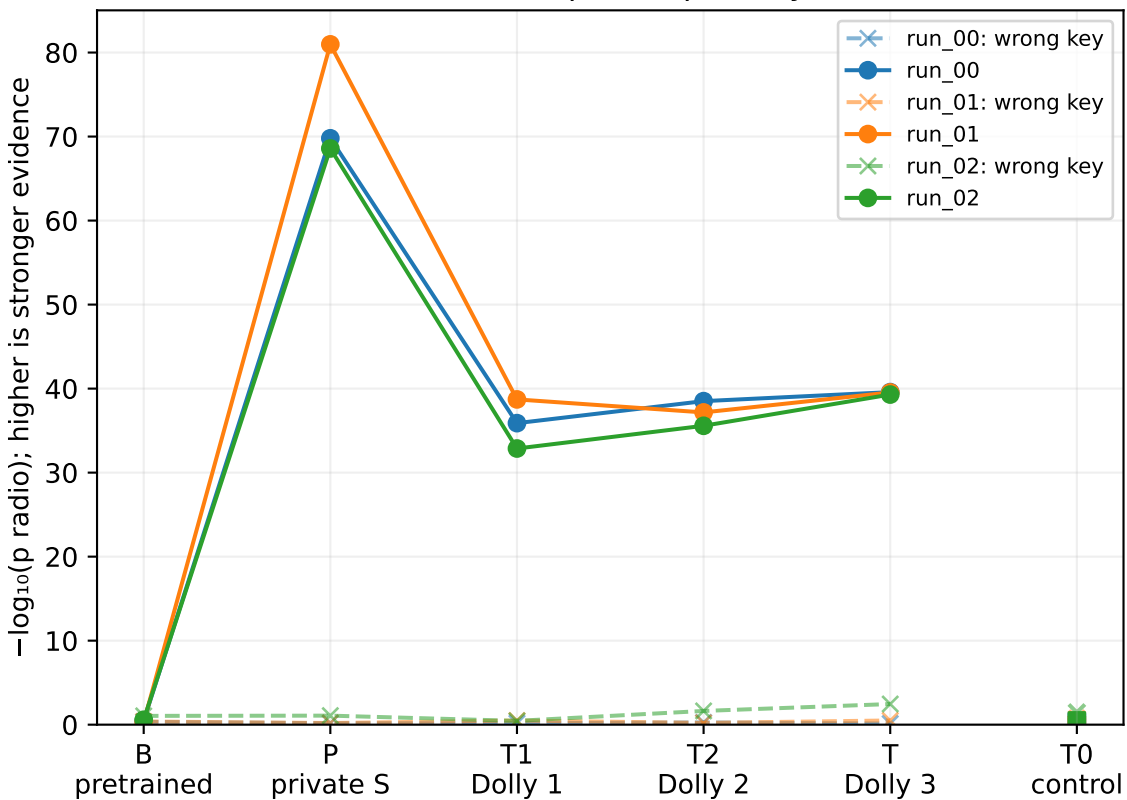
Unseen S' probe (primary)
