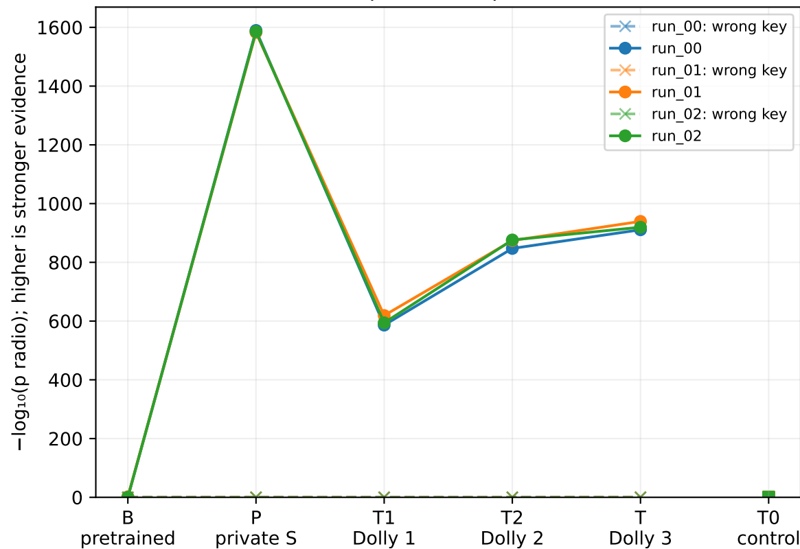
Supervised S probe
