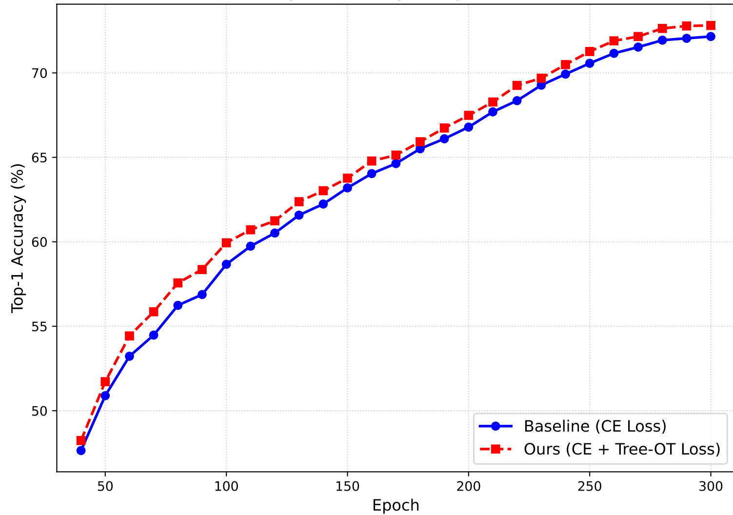
Top-1 Accuracy Comparison
