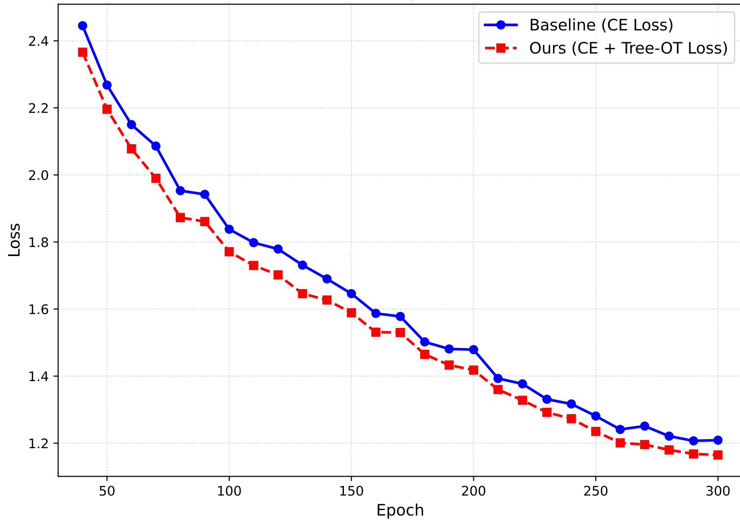
Loss Comparison
