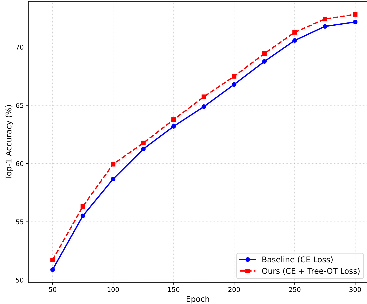
Top-1 Accuracy Comparison
