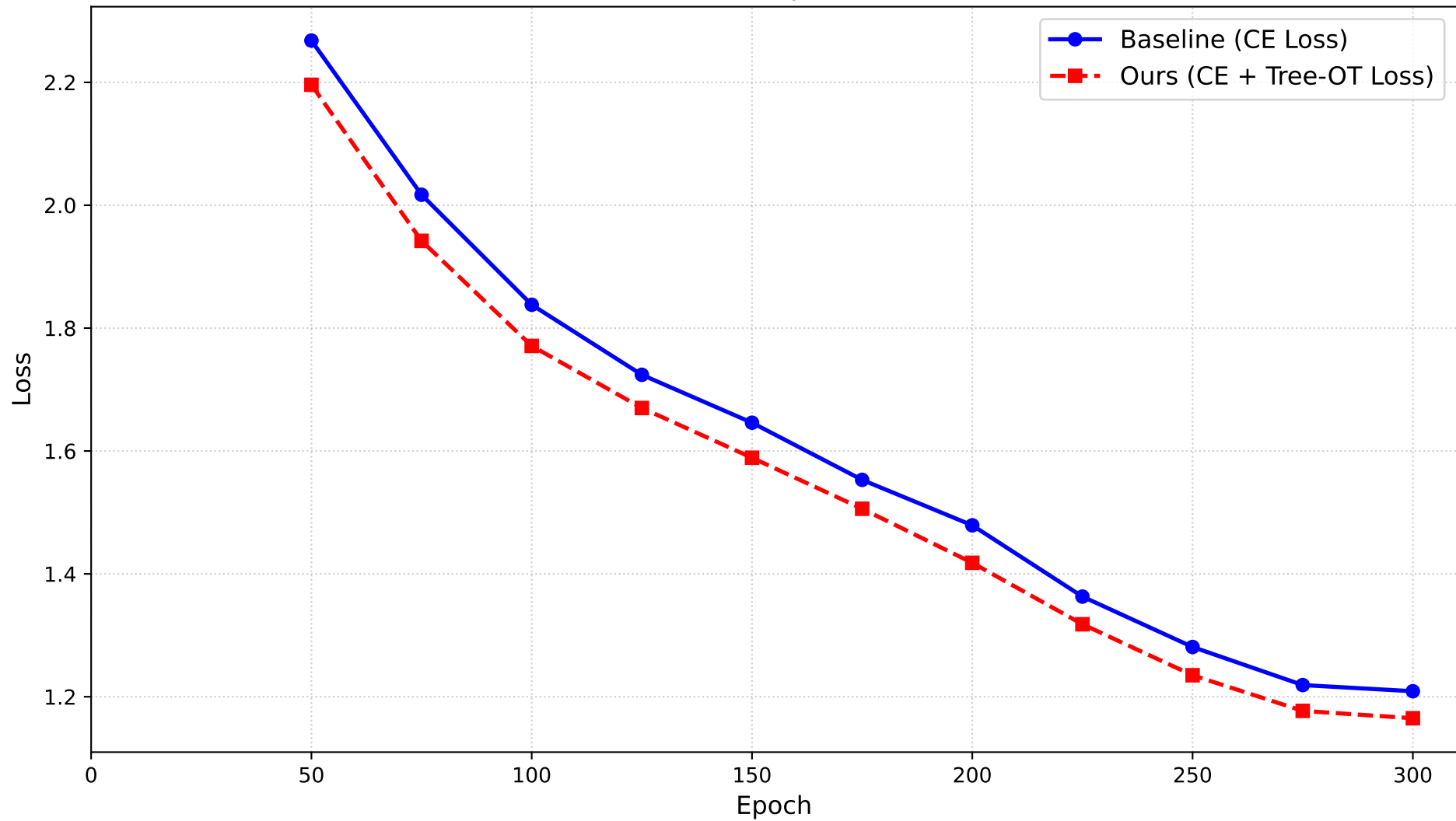
Loss Comparison
