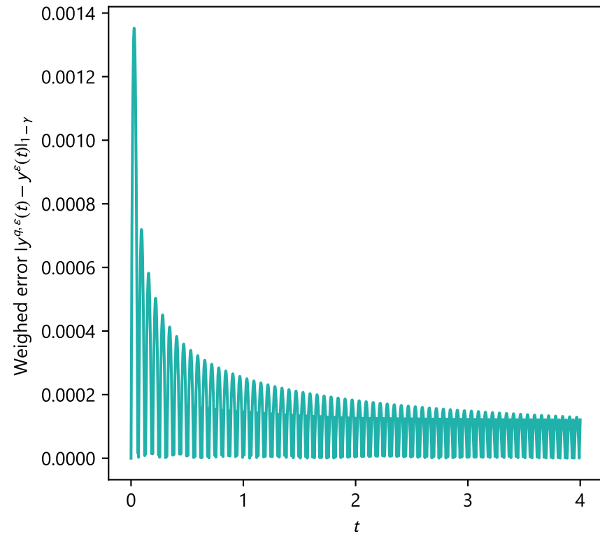
Absolute weighed error over time h = 2^{-4}
