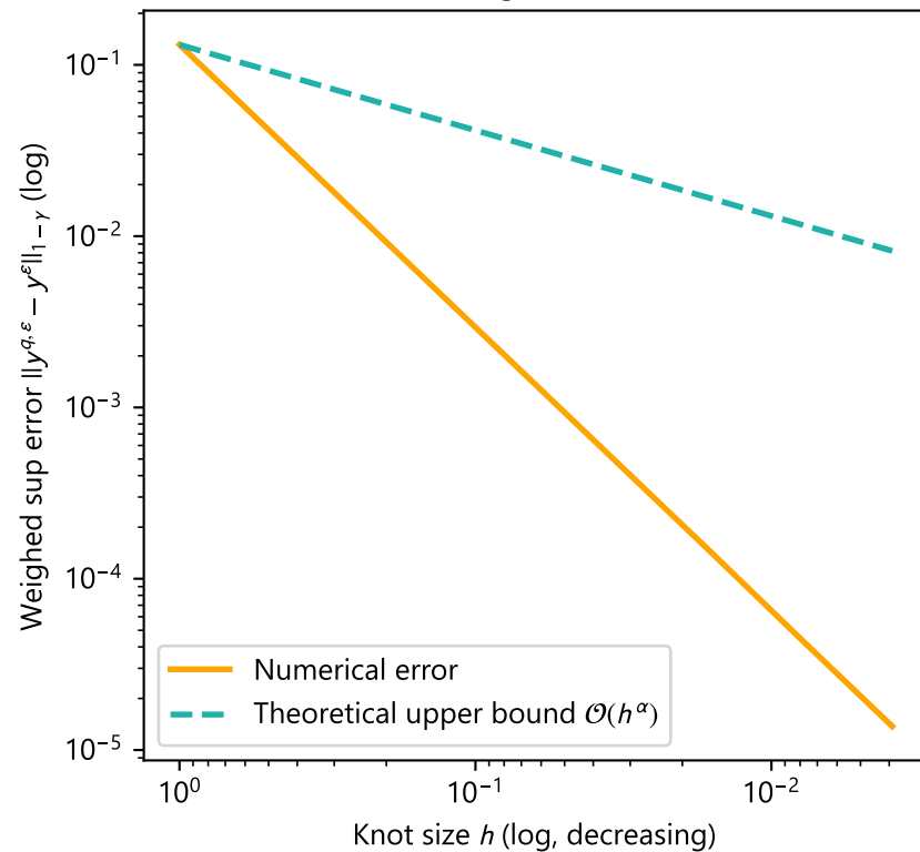
Convergence order
