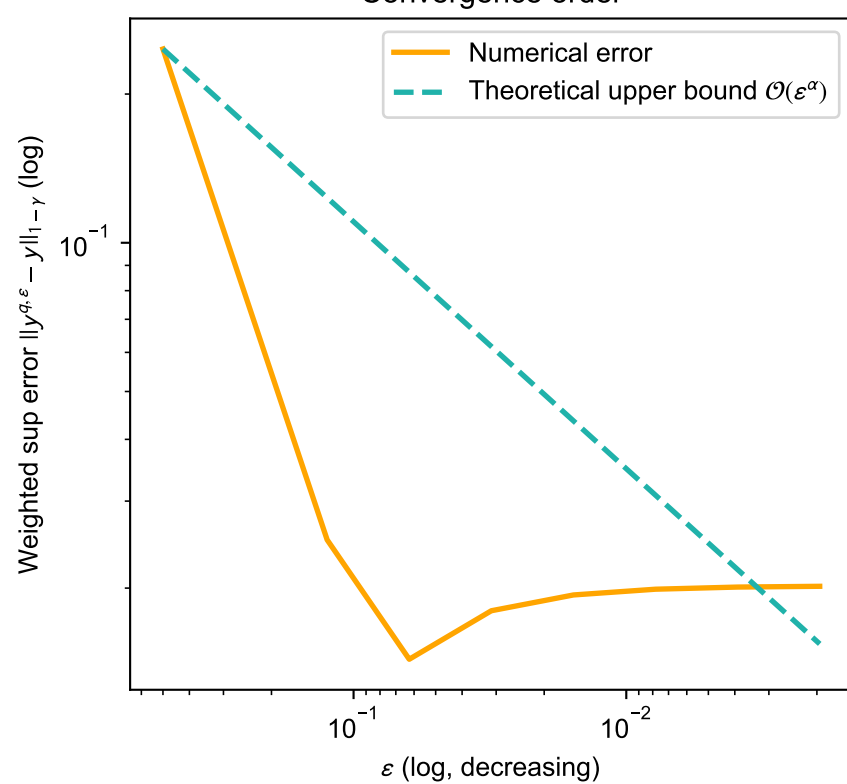
Convergence order
