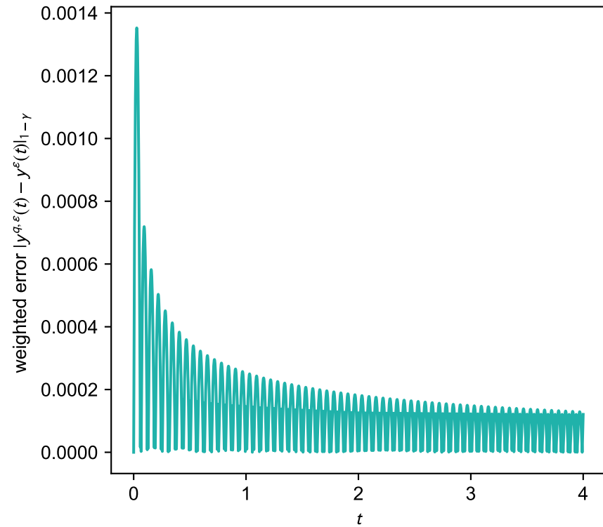
Absolute weighted error over time h = 2^{-4}
