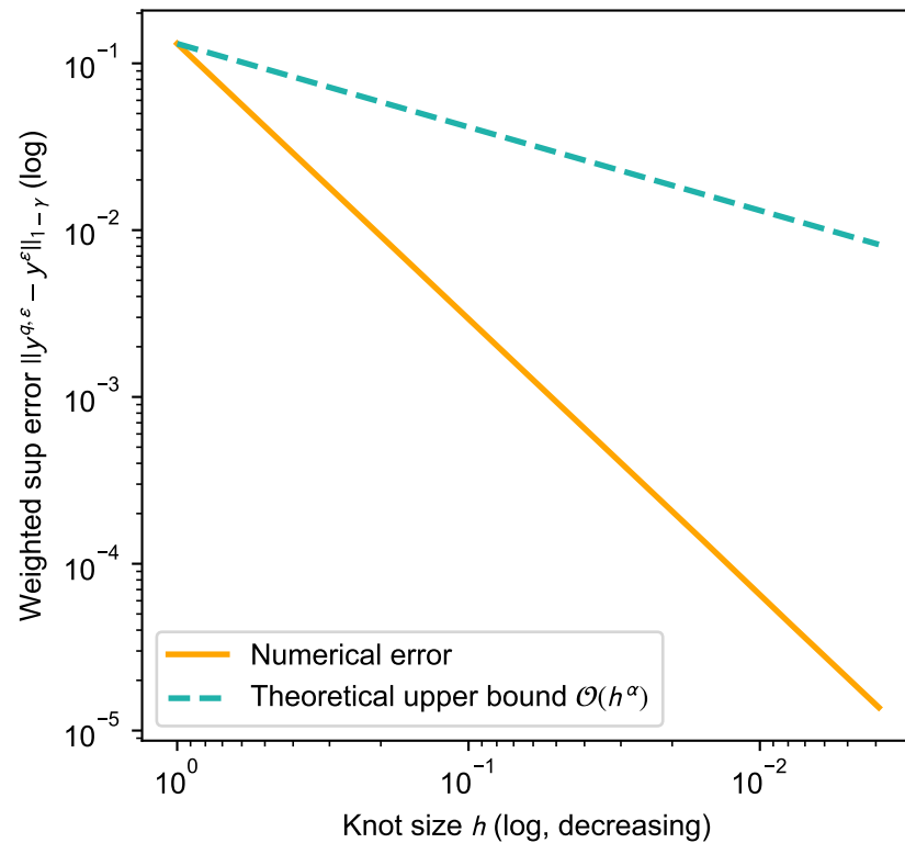
Convergence order
