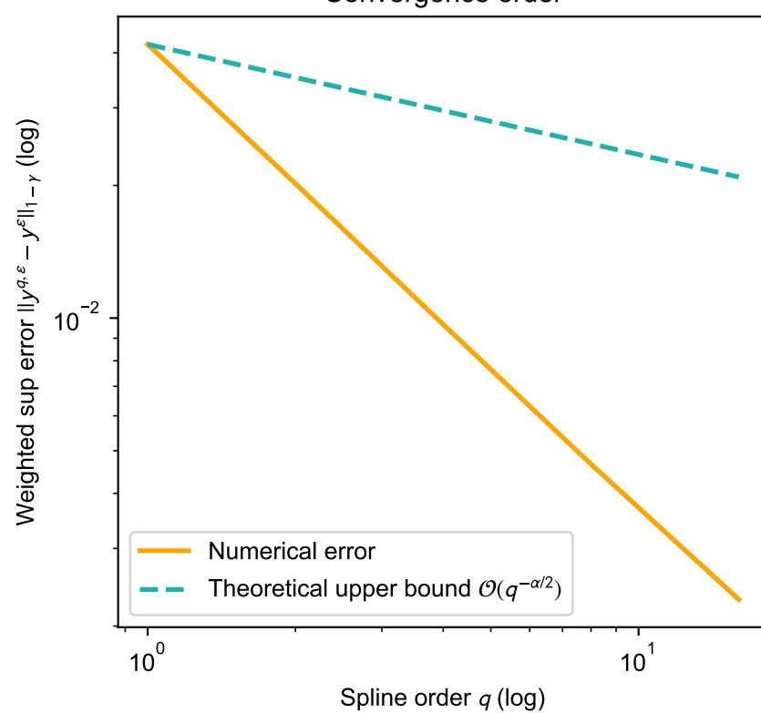
Convergence order
