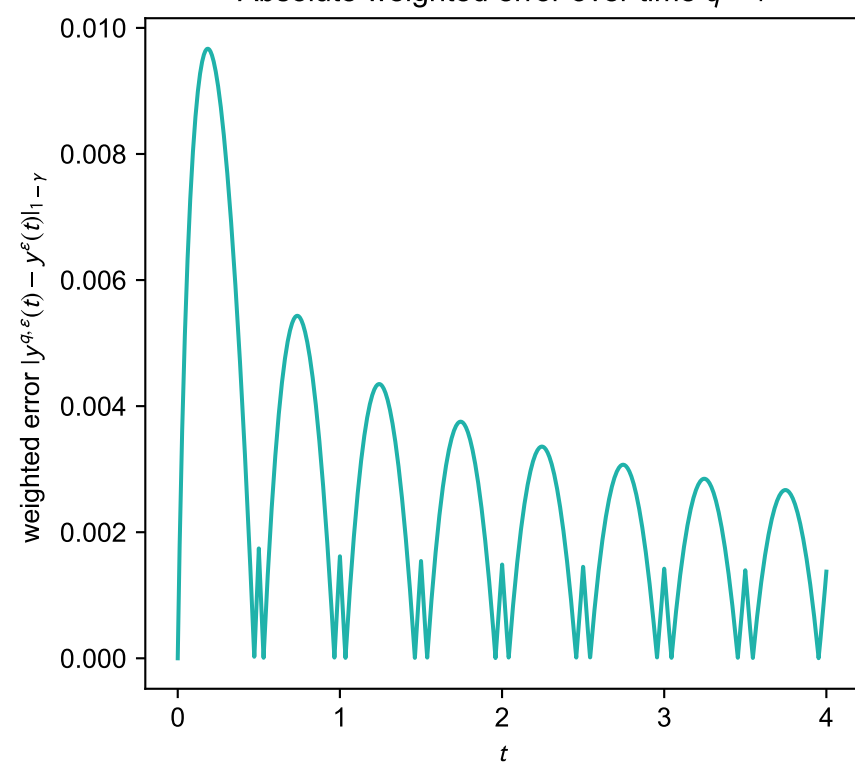
Absolute weighted error over time q=4
