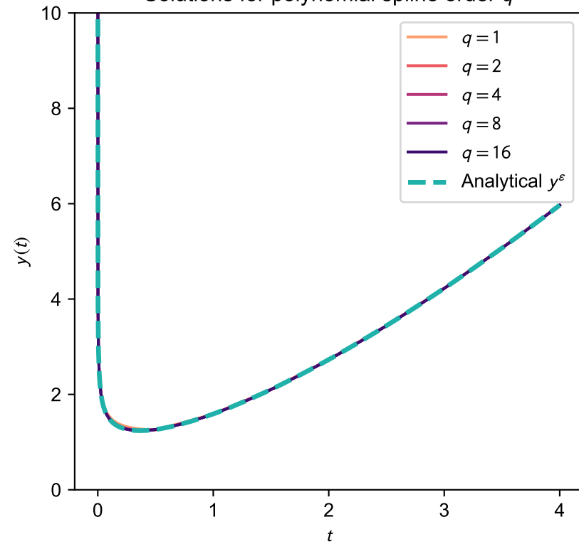
Solutions for polynomial spline order q
