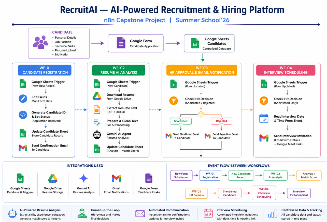
Figure 1. Overall RecruitAI architecture and event flow.
