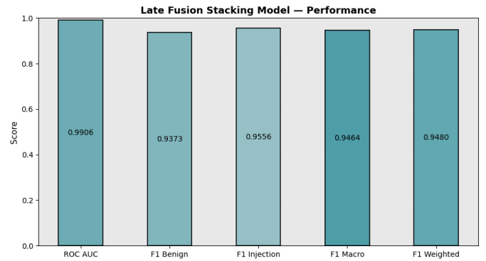
Fig. 6. Bar Graph of Combined Late Fusion Model's performance comparison over five metrics ROC-AUC scores, F1 Benign, F1 Injection, F1 Macro-averaged scores, and F1 weighted-averaged scores, illustrating classification performance and class-balance sensitivity across different evaluation metrics.
