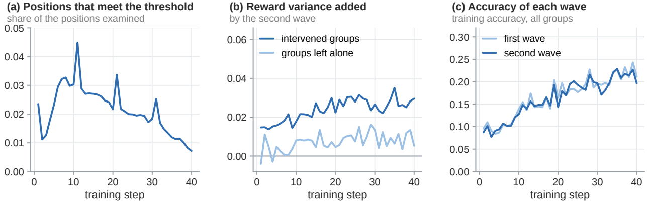
Figure 6. Three measurements of the second wave on Video-HopChain, over the training steps. The left panel gives the share of the positions the mask examines whose top-1 probability exceeds \tau , whereas the middle panel gives the reward variance the second wave adds to a group, both on the intervened groups and on the groups the mask leaves alone, which already carry variance in their first wave. The right panel then gives the training accuracy of each wave over all groups.
