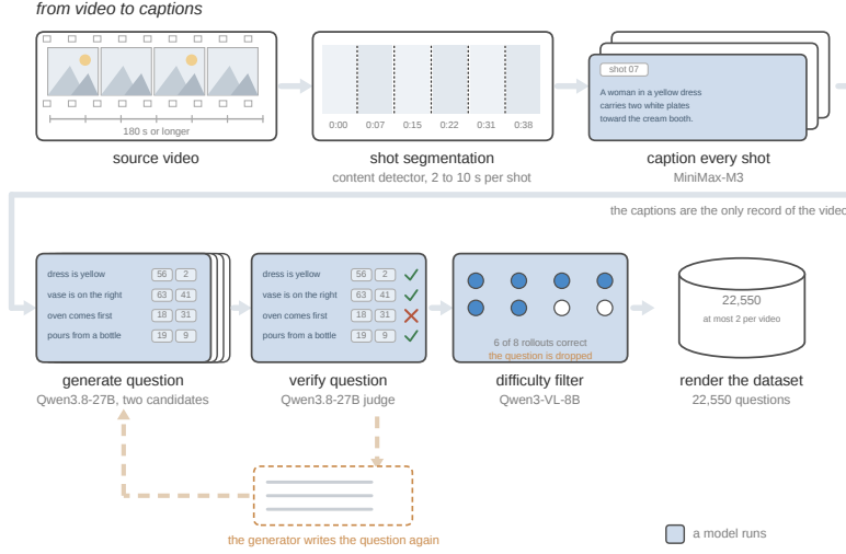
Figure 4. The Video-HopChain generator.
