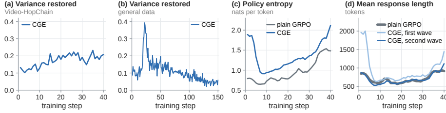
Figure 3. Four training metrics of our runs, over the training steps.
