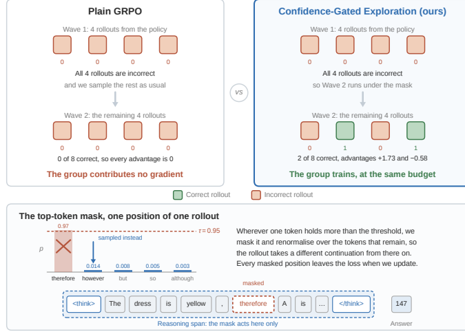
Figure 2. Confidence-Gated Exploration on one group of G rollouts.
