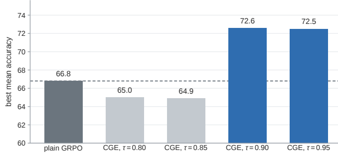
Figure 5. Best mean accuracy over the six image benchmarks of OpenMMReasoner, for plain GRPO and for CGE at four thresholds. The dashed line marks plain GRPO, and the two grey bars are the runs that never learn the answer format.
