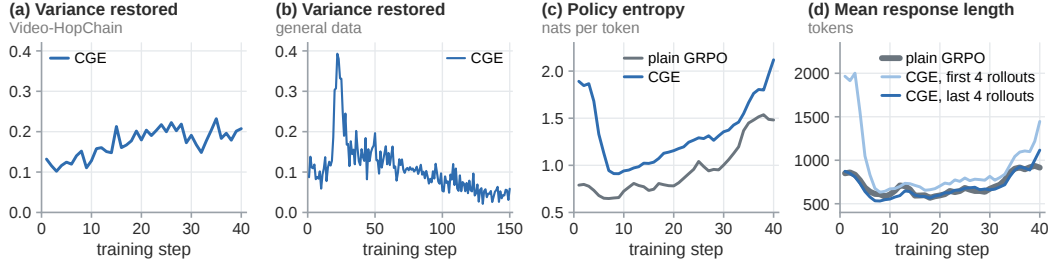
Figure 5: Four training metrics of our runs, over the training steps.
