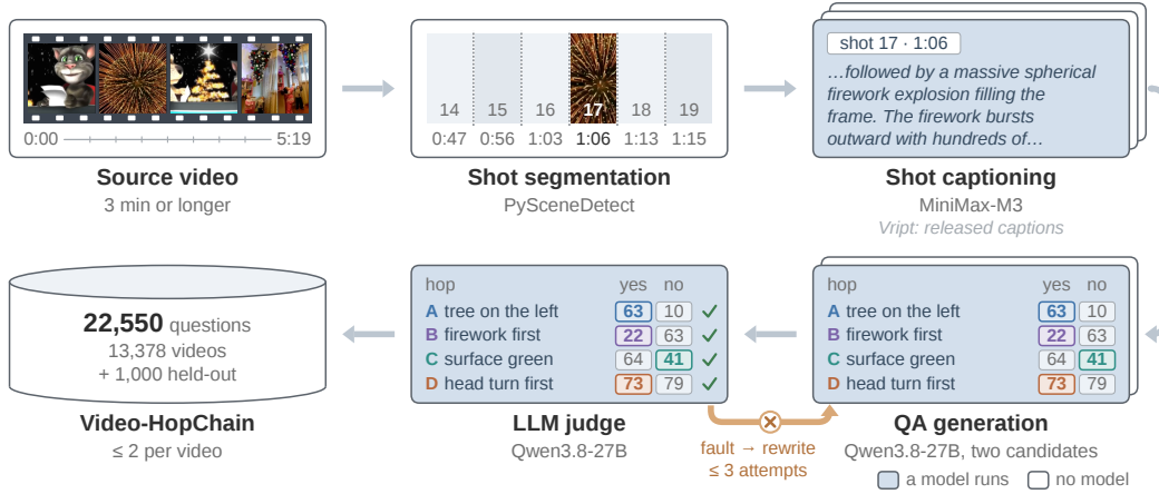
Figure 3: The Video-HopChain generator.
