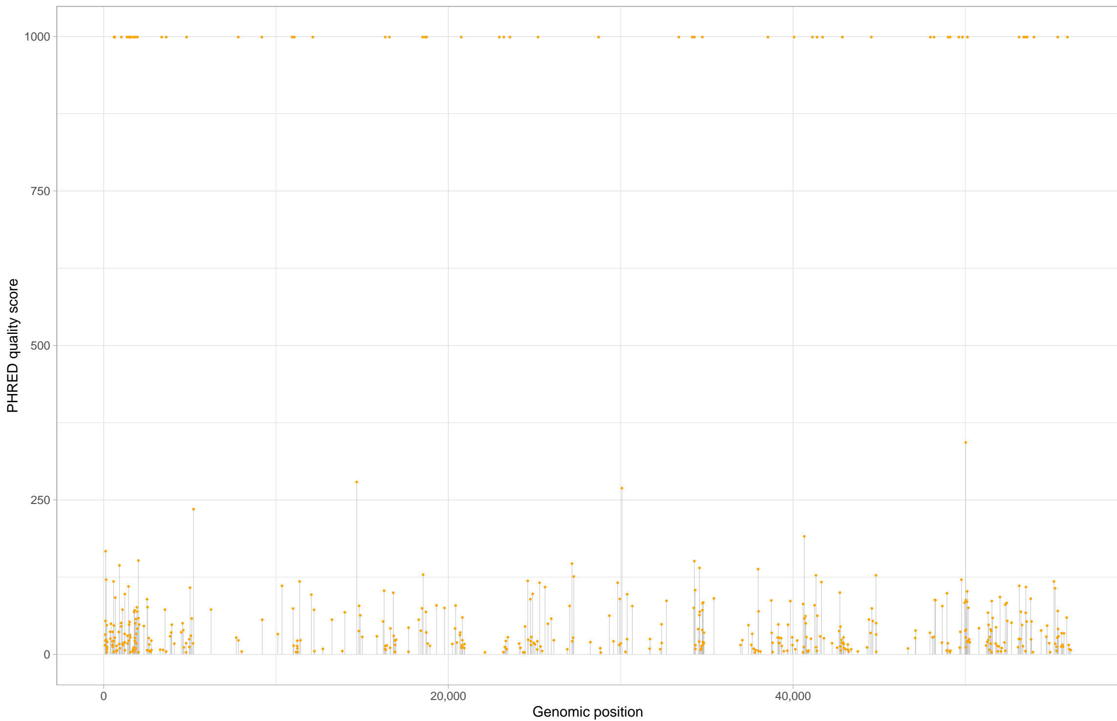
Chromosome chr4_random
