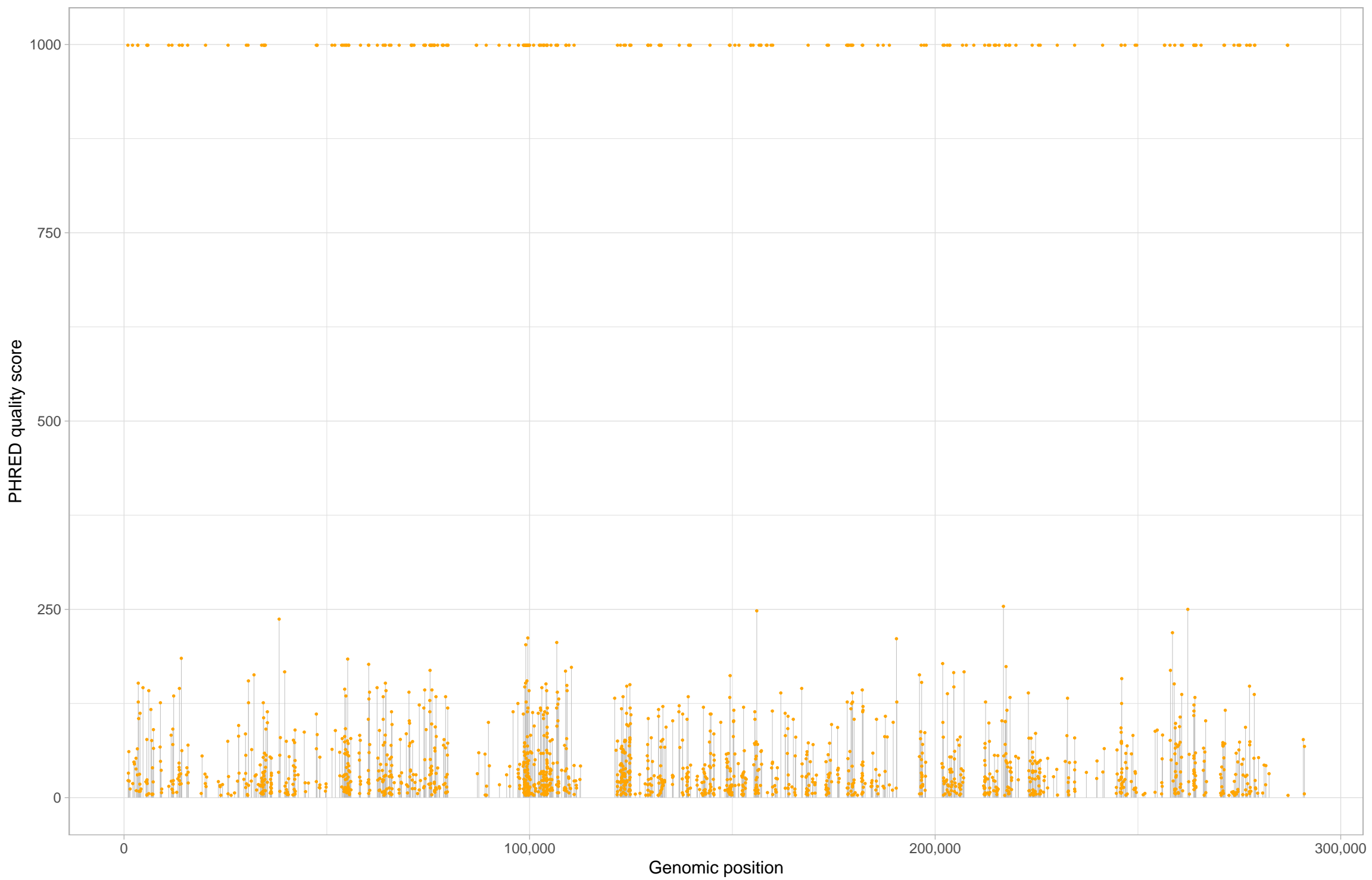
Chromosome chr26
