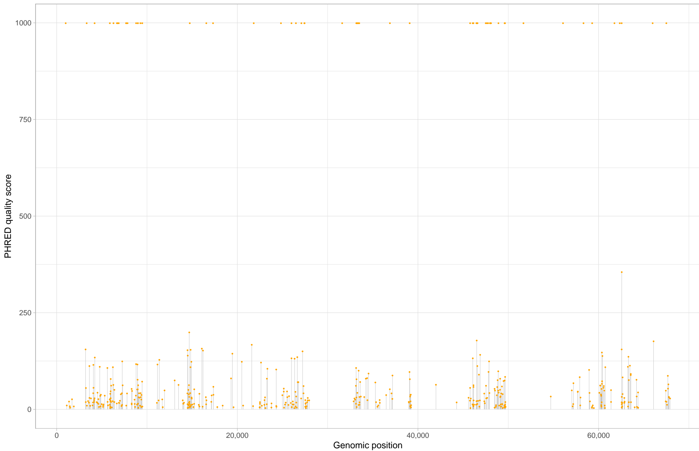
Chromosome chr1B
