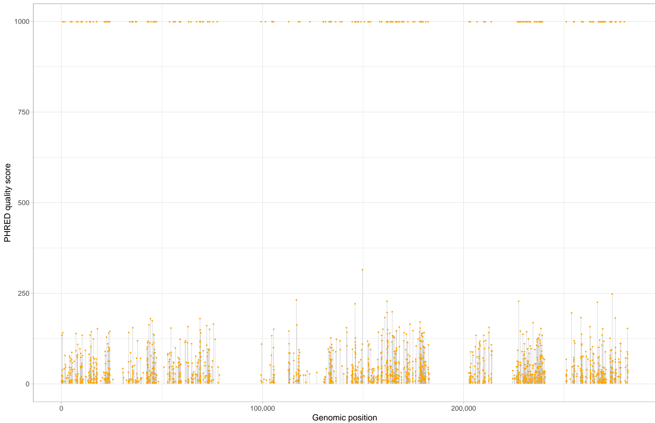
Chromosome chr27
