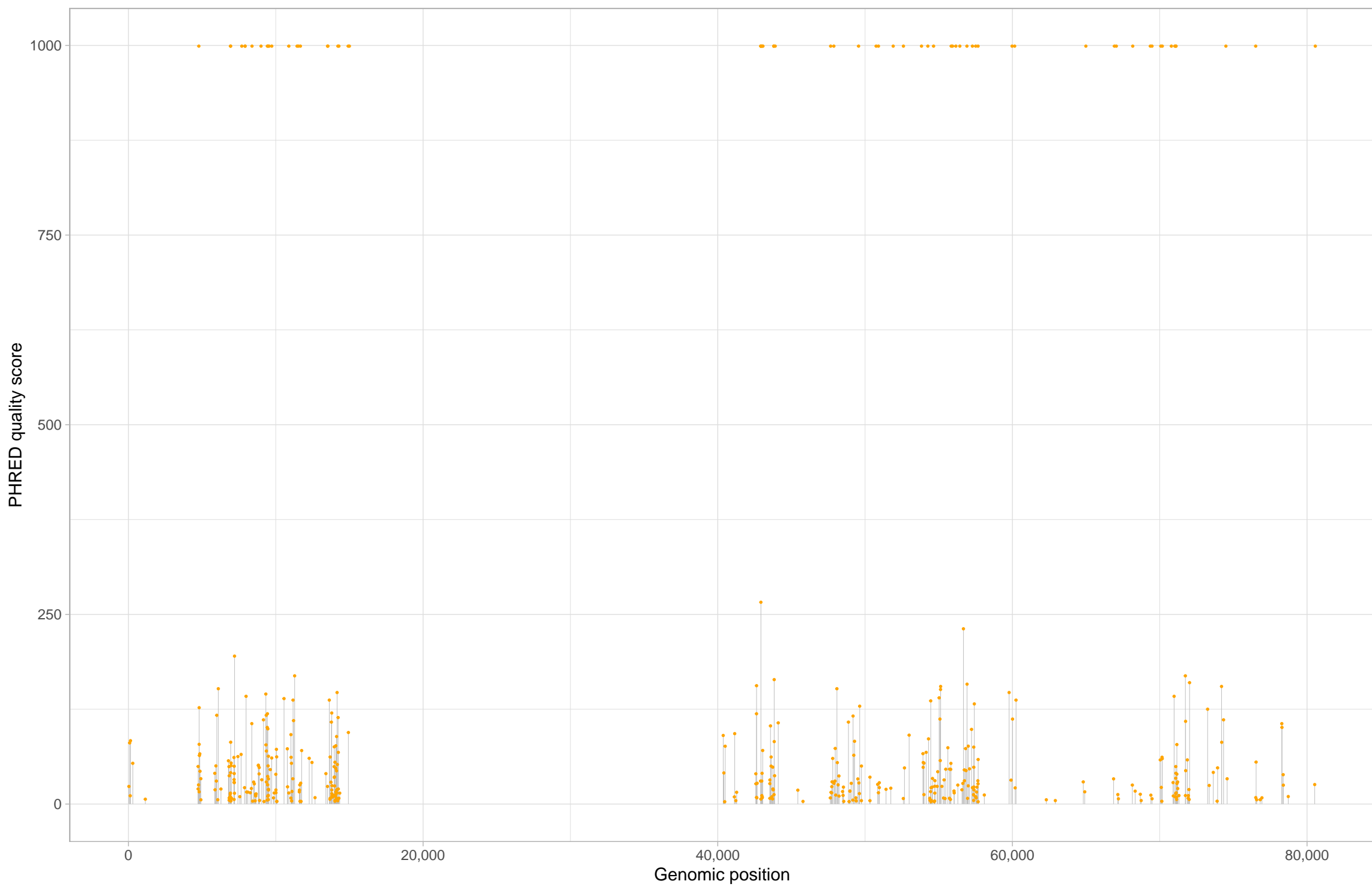
Chromosome chr3_random
