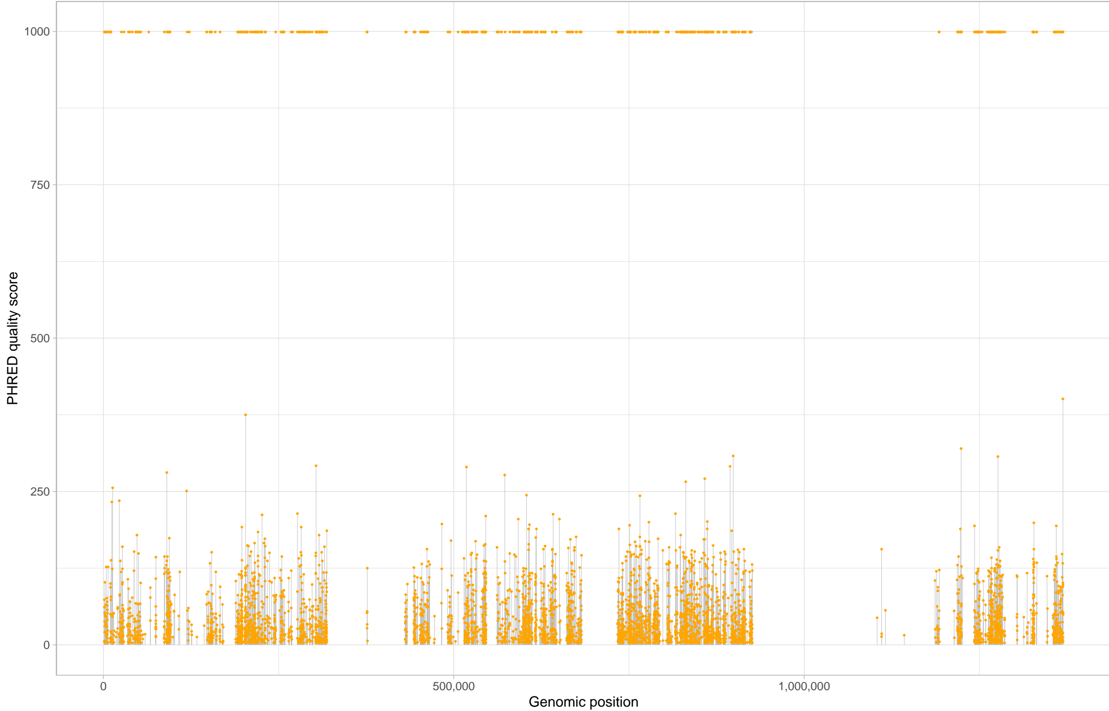
Chromosome chr18
