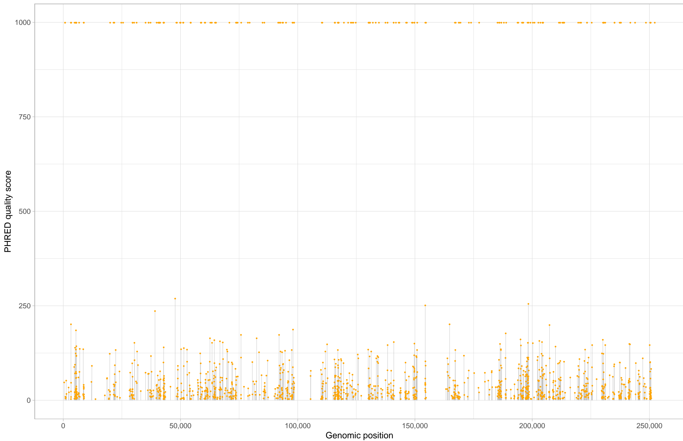
Chromosome chr24
