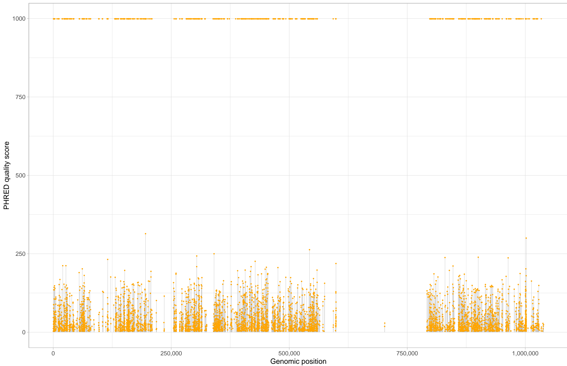
Chromosome chr19
