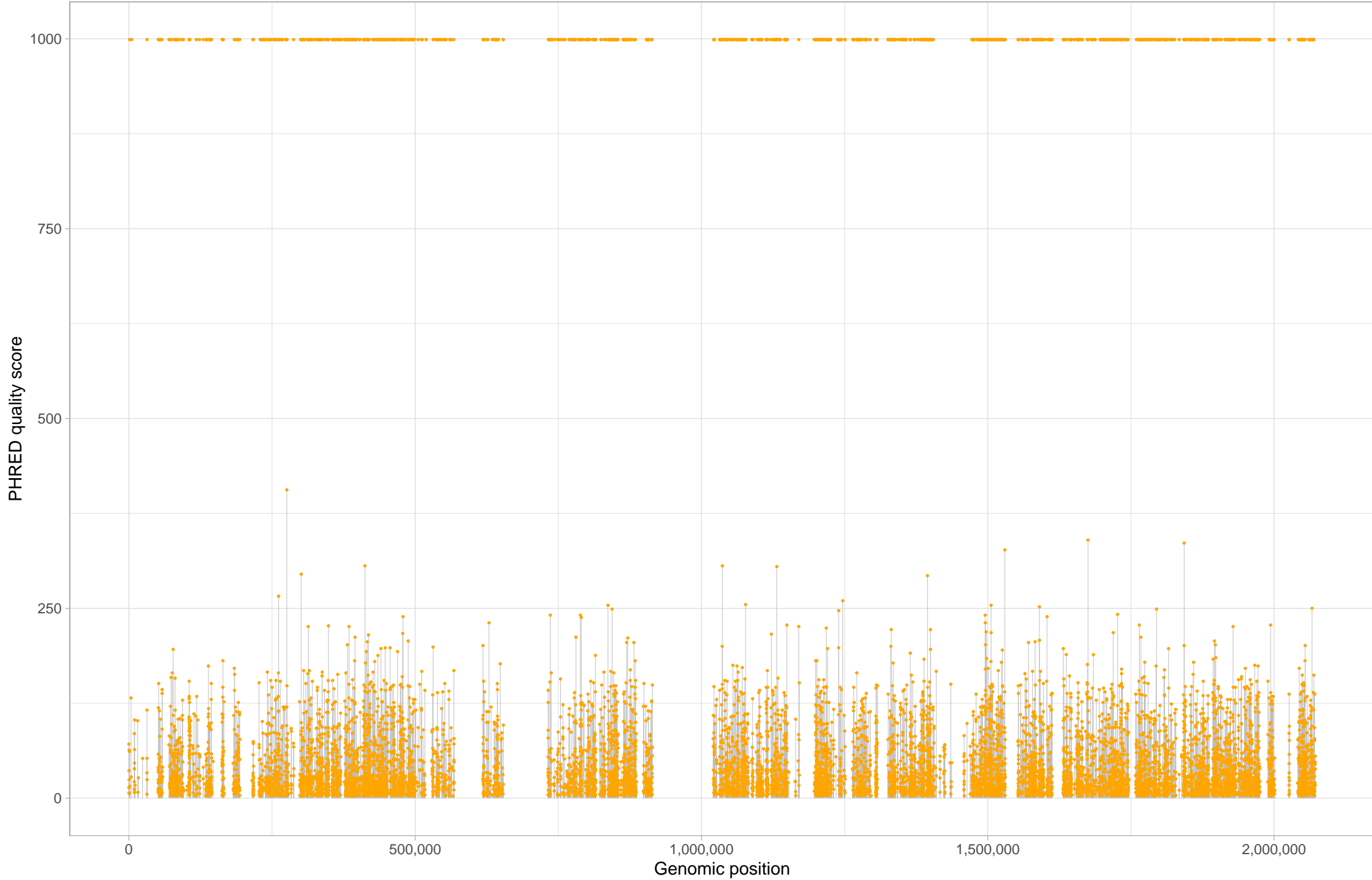
Chromosome chr9
