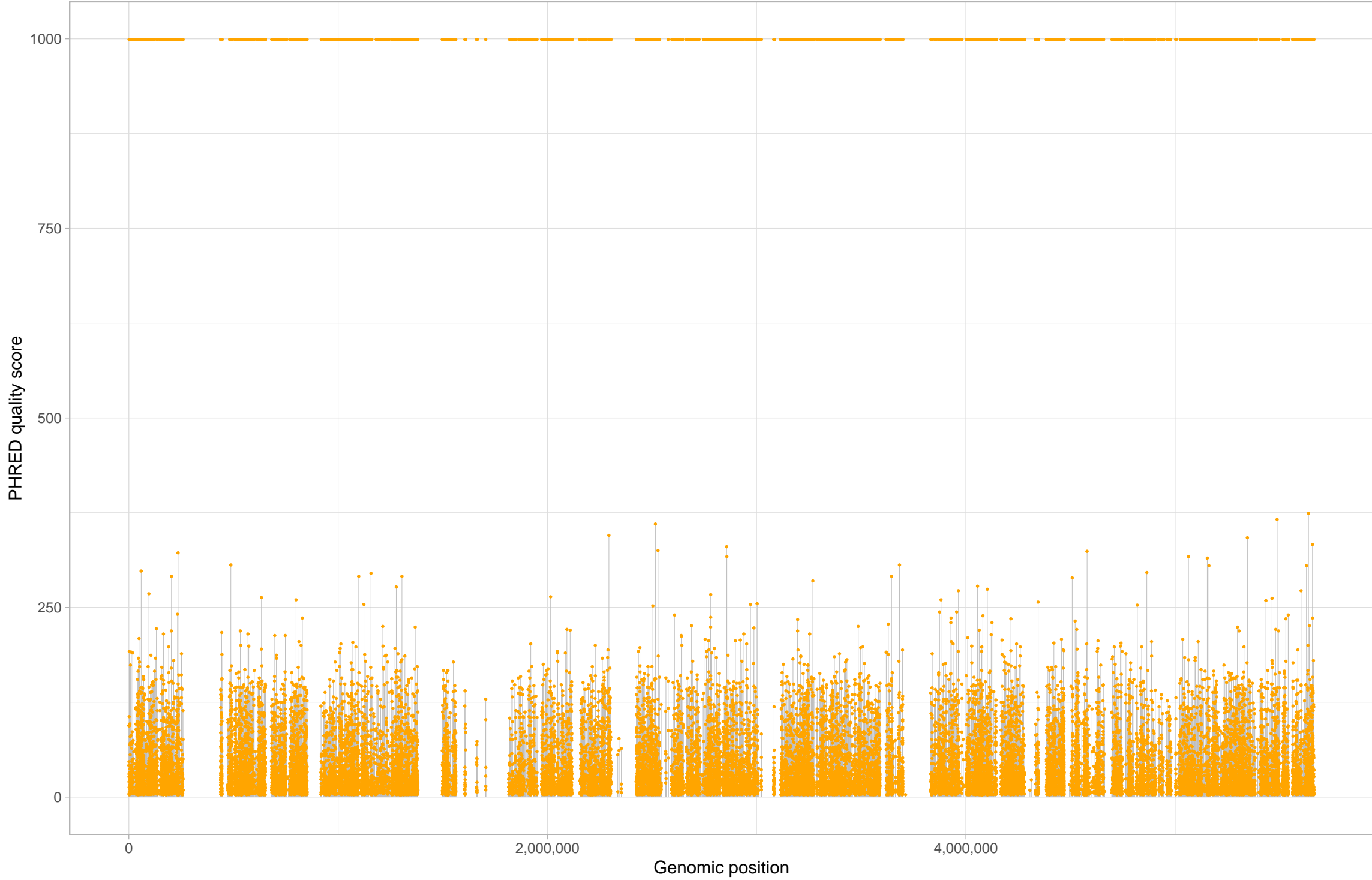
Chromosome chr5
