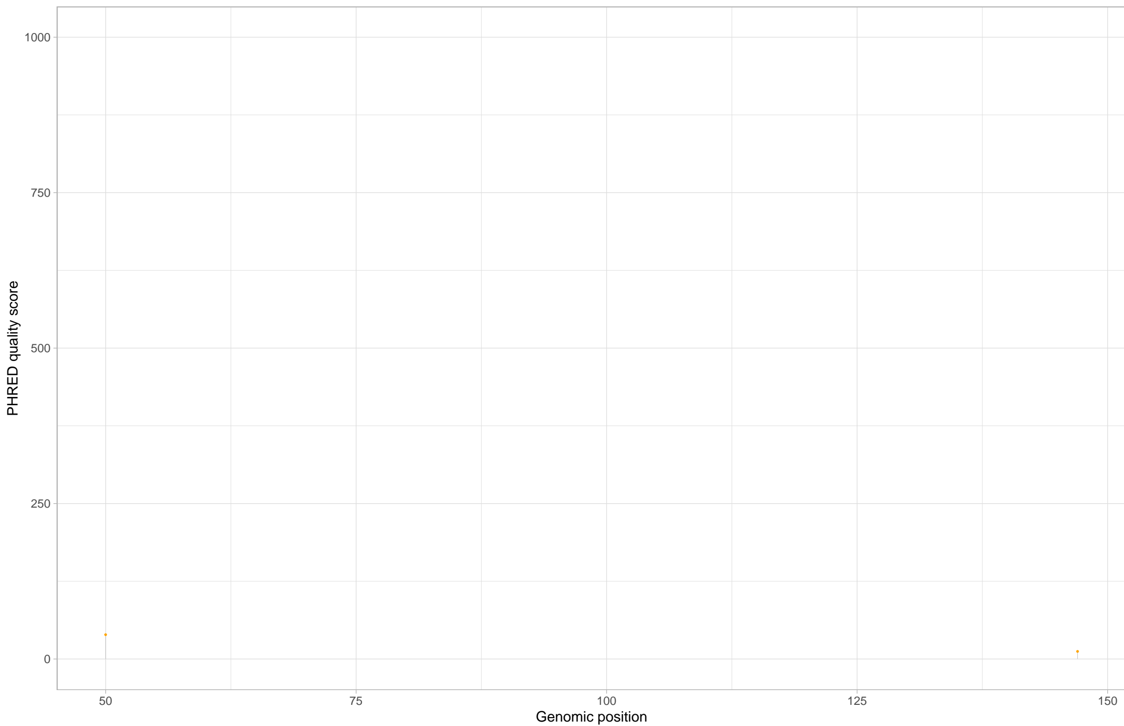
Chromosome chr11_random
