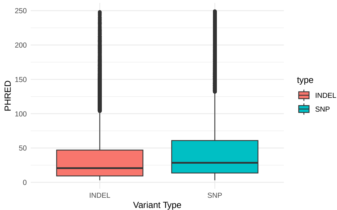
PHRED Quality by Variant Type
