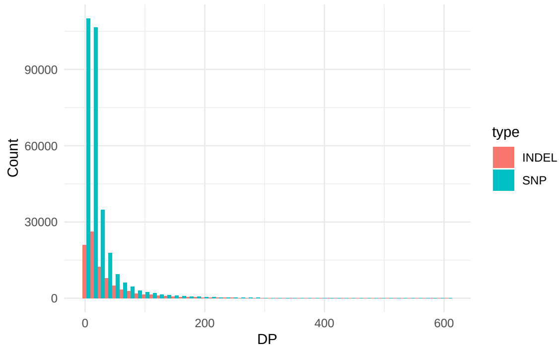
Read Depth (DP): INDEL vs SNP
