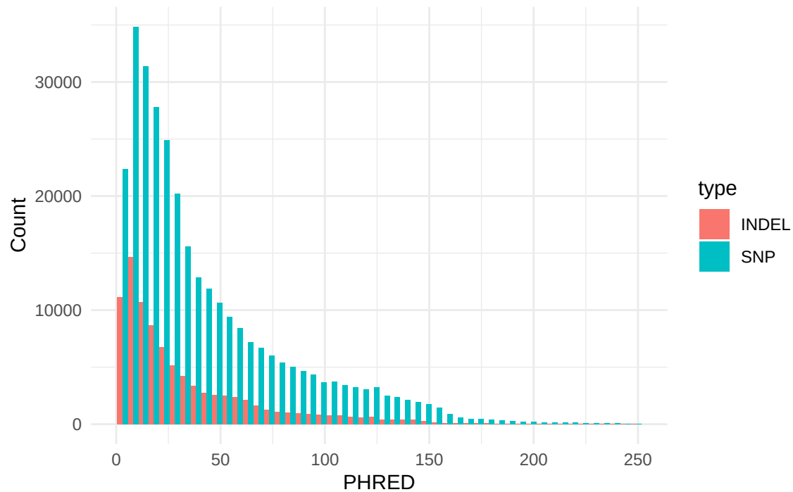
PHRED Quality: INDEL vs SNP
