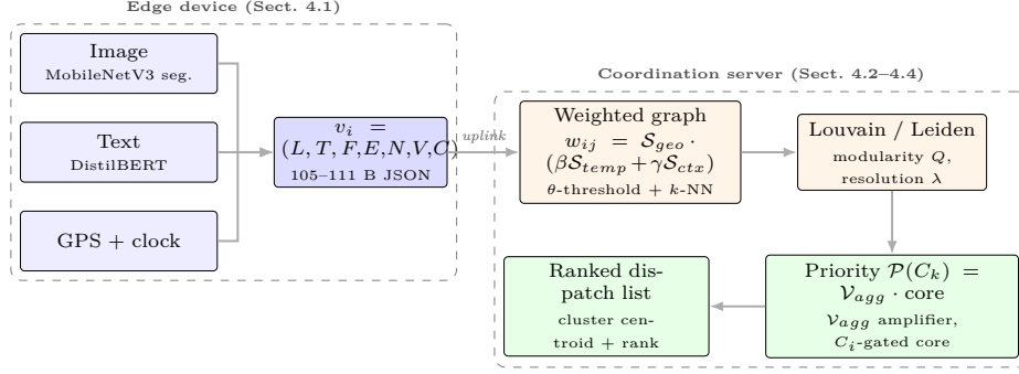
Fig. 1. End-to-end architecture. The edge device compresses raw multimedia into a 105–111-byte attribute vector; the server builds the gating weighted graph, decomposes it into operational zones, and ranks them. Only the metadata packet crosses the degraded link.
