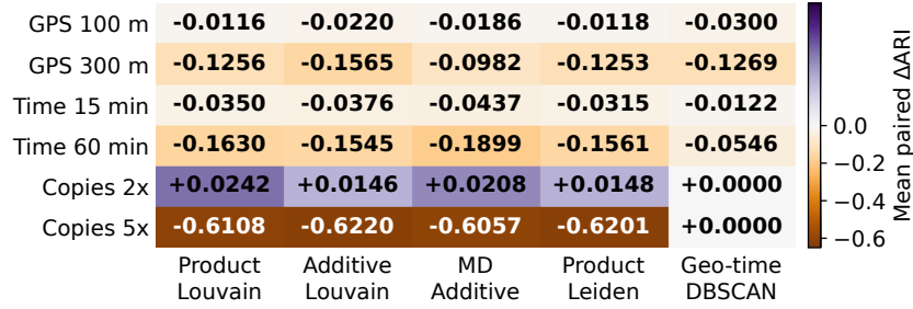
Fig. 2. Mean paired change in RQ1 ARI relative to each method’s control over 40 held-out runs. Cells use original incident-linked reports; negative values indicate degradation; MD Additive denotes matched-density Additive. Intervals are not shown and no between-method test is implied.
