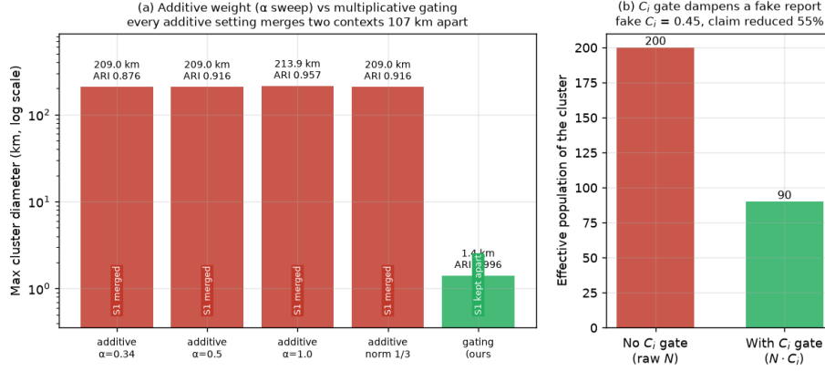
Fig. 2. (a) Worst-case cluster diameter (log scale) for the four additive settings and gating; every additive setting merges the two S1 contexts 107 km apart, while gating keeps them separate. (b) The confidence gate reduces the fake report’s claimed population of 200 to an effective 90—a 55% reduction of phantom population.
