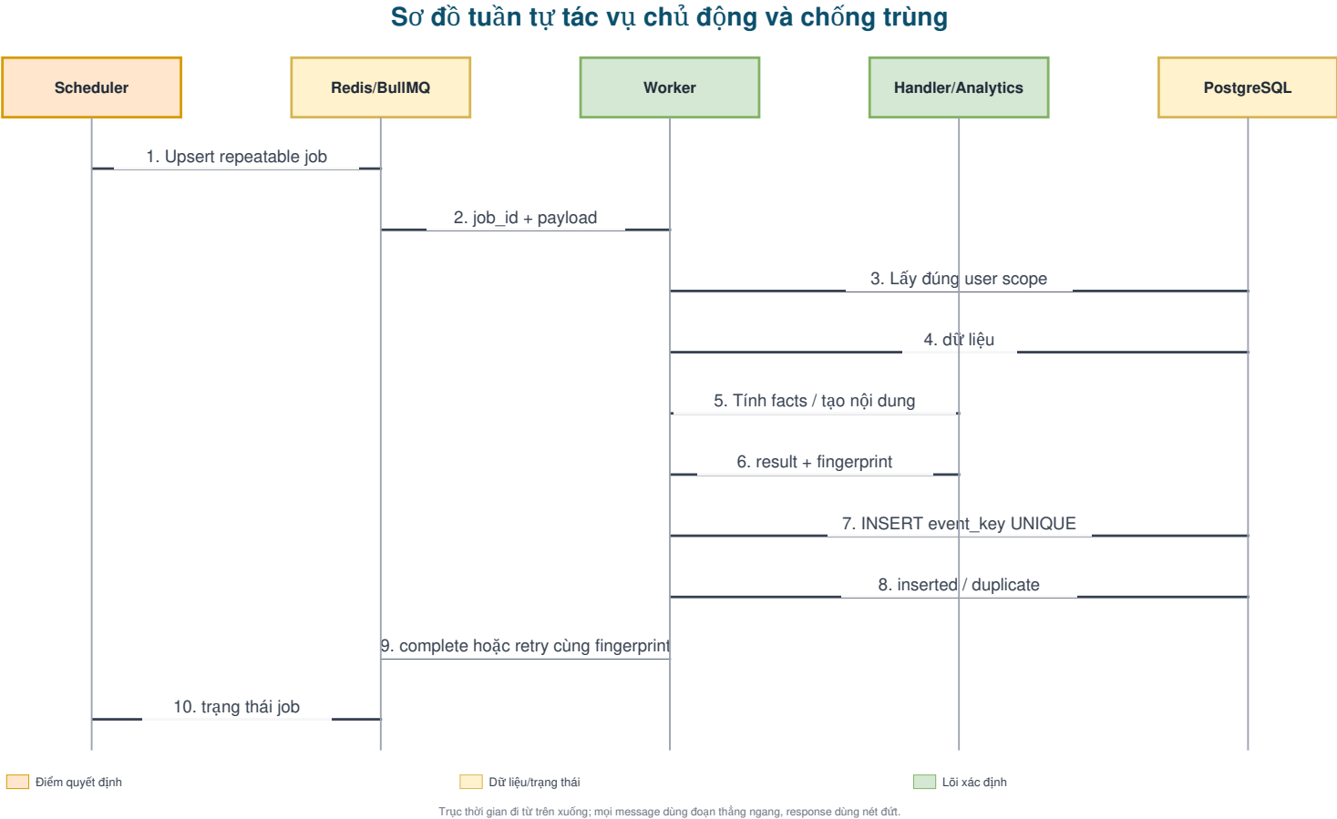
Figure 13: Sequence diagram for proactive tasks and the mechanism preventing duplicate effects on retry.
