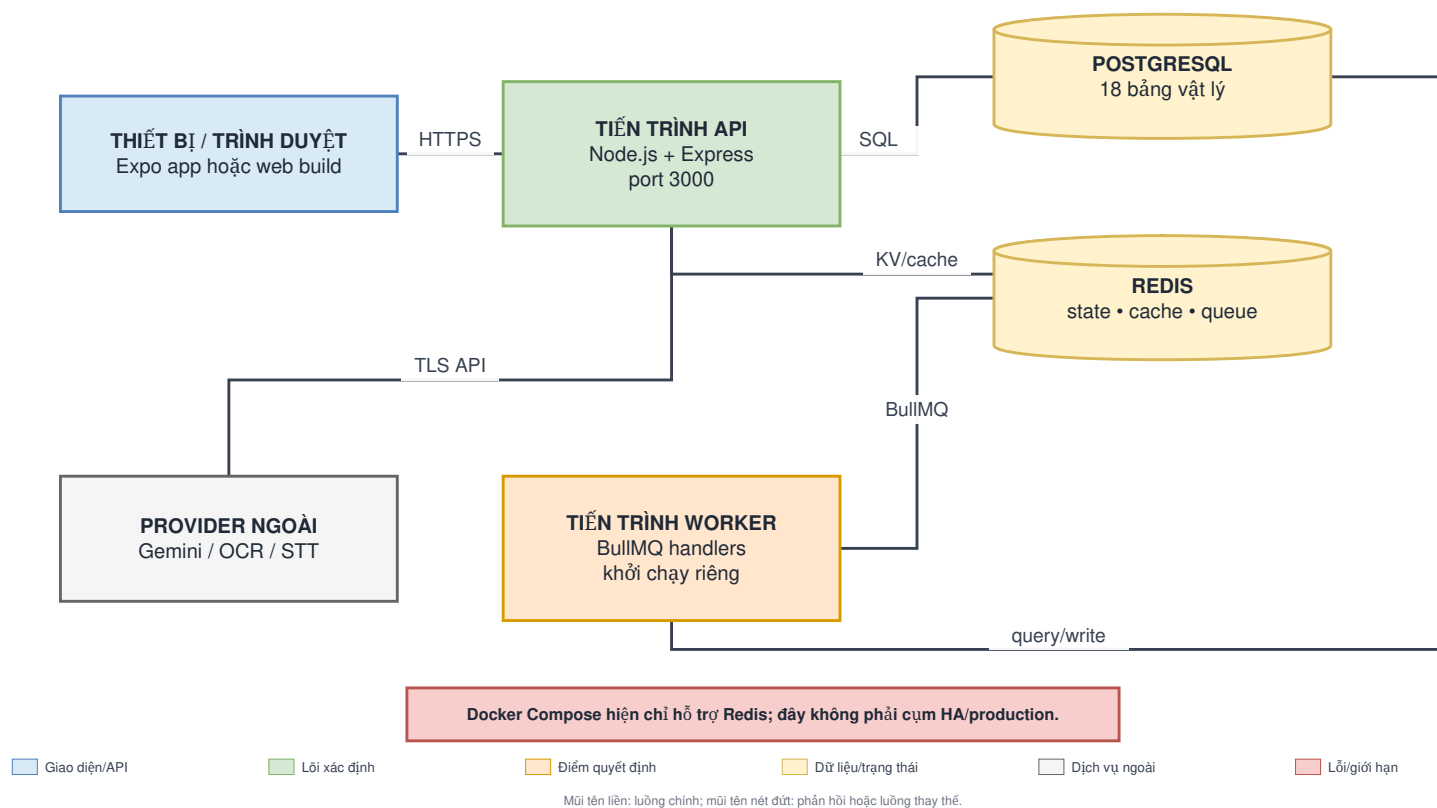
Figure 3: Prototype deployment diagram. The frontend, API, worker, PostgreSQL and Redis belong to the demo environment; the AI provider is called over the network.
