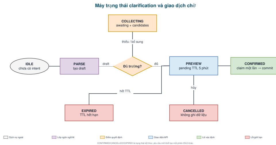
Figure 7: The conversation and pending-transaction state machine.
