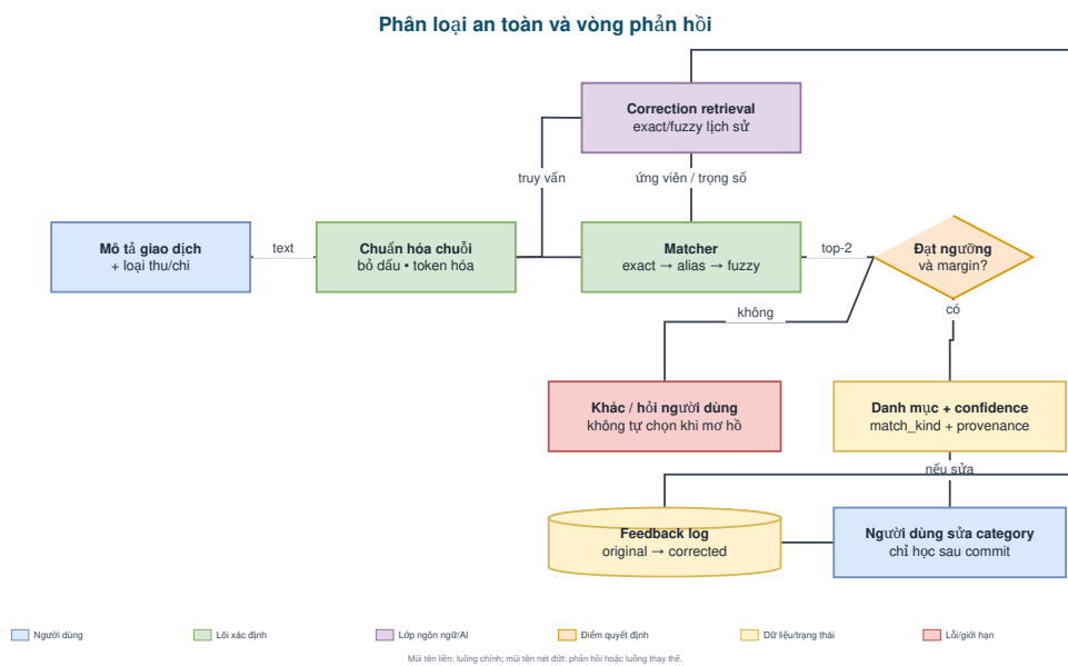
Figure 10: The classification feedback and personalization flow using correction retrieval, not fine-tuning.
