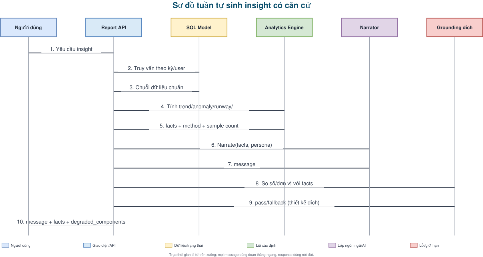
Figure 11: Sequence diagram for grounded insight generation. The response returns both the message and the facts for traceability.
