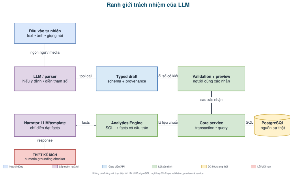
Figure 6: The LLM’s responsibility boundary: data and facts are created in the deterministic core; the LLM only performs semantic conversion and interpretation.
