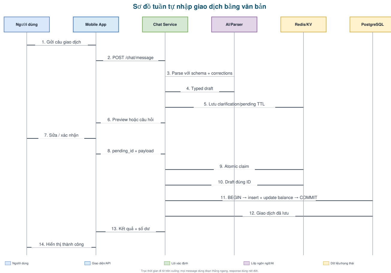
Figure 8: Sequence diagram for text transaction entry. The LLM sits outside the data-writing transaction.
