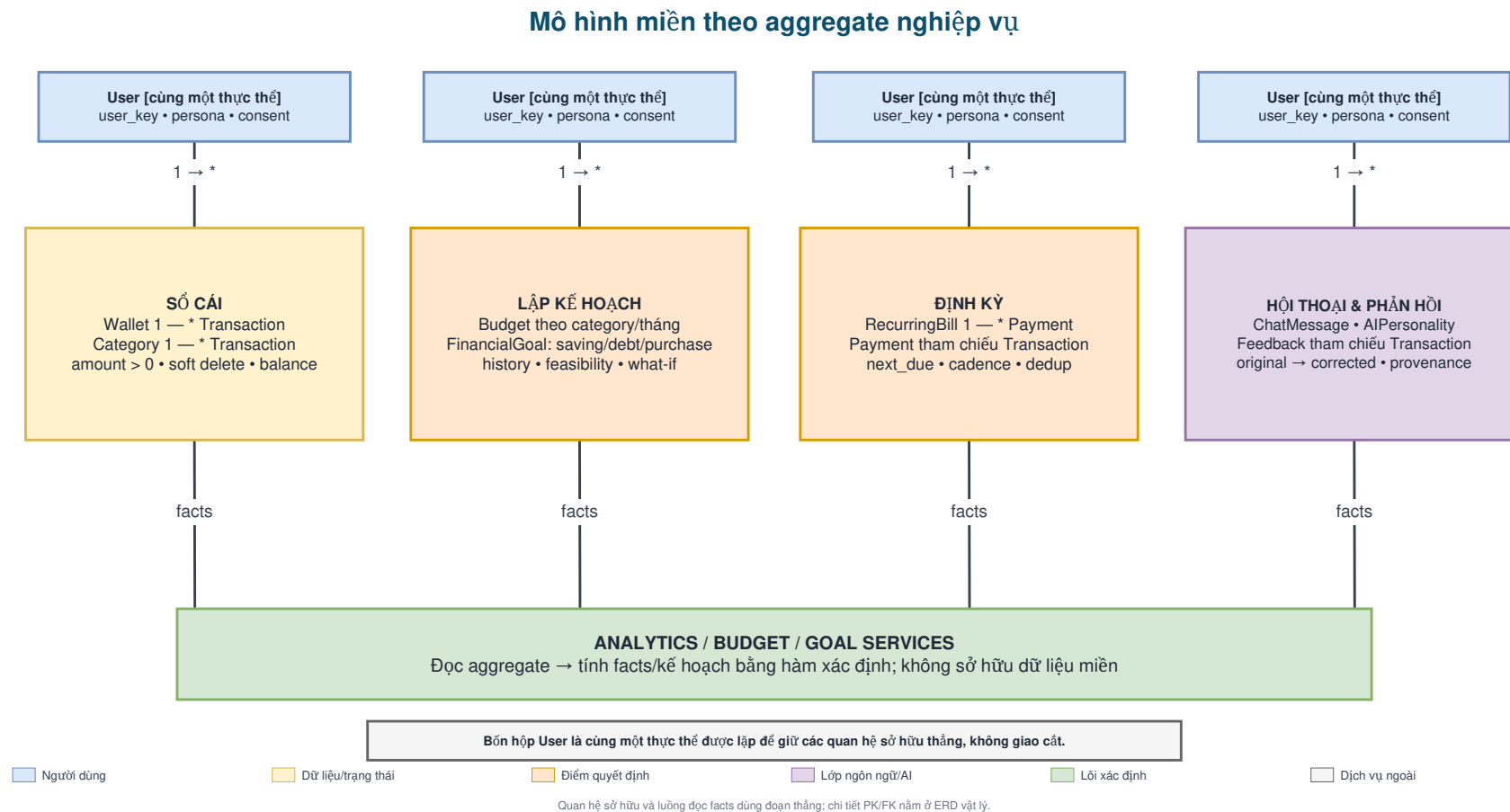
Figure 4: Domain model by business aggregate. The data clusters are separated from the analytics services and the language layer.
