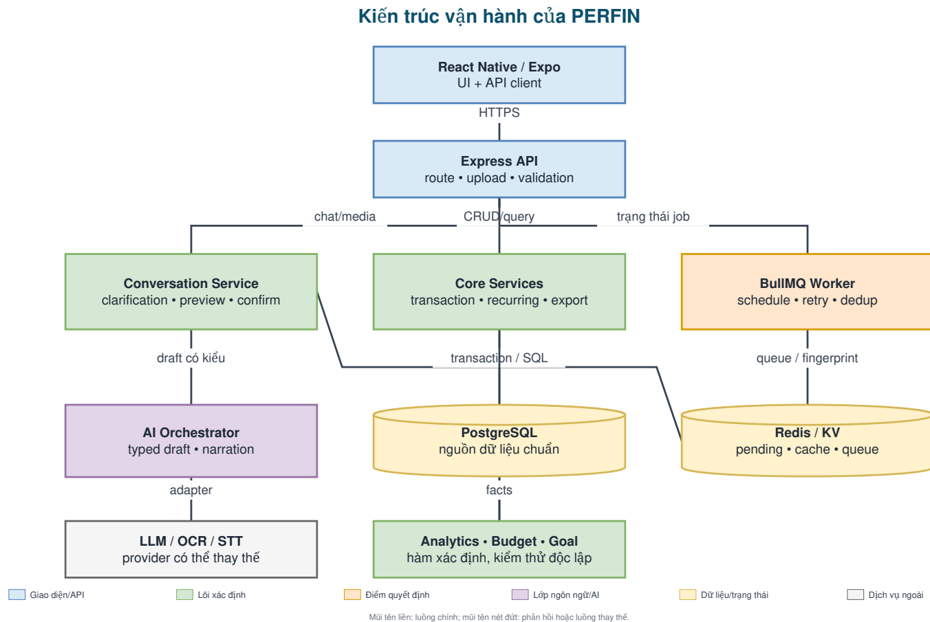
Figure 2: PERFIN’s runtime architecture. The deterministic core creates and stores facts; the AI Orchestrator only coordinates semantics.
