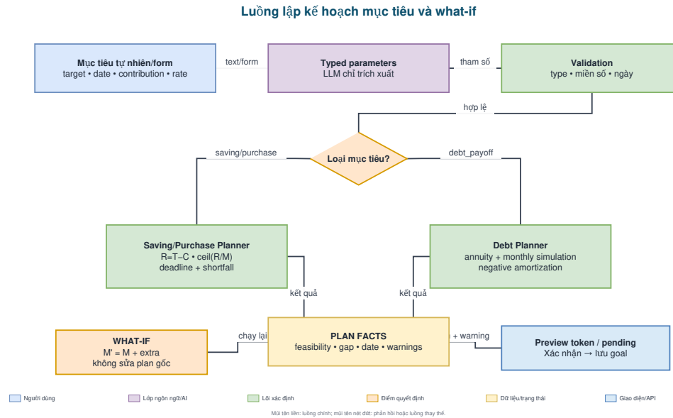
Figure 12: The goal-planning and what-if simulation flow.
