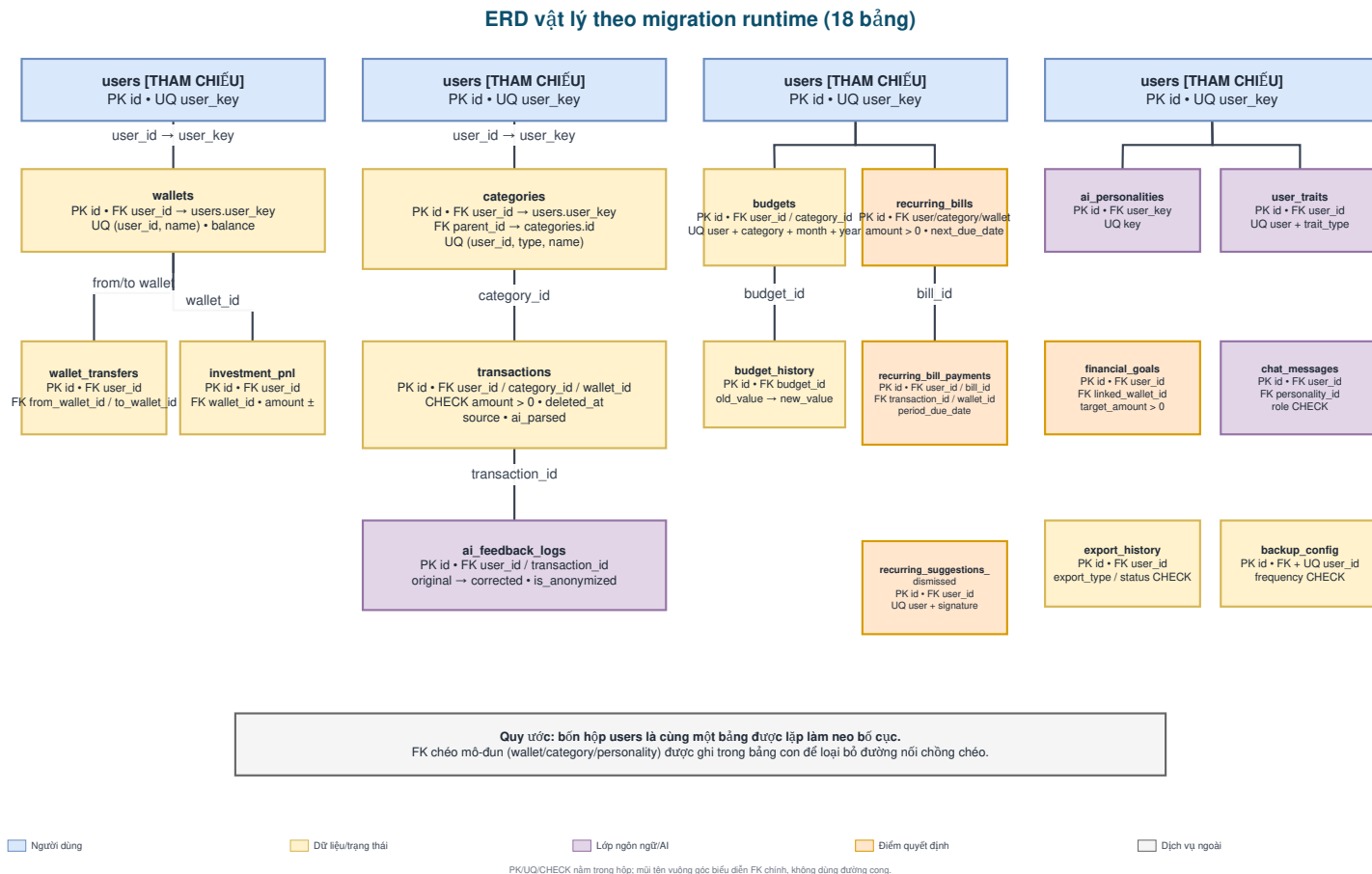
Figure 5: The physical entity–relationship diagram reconciled with the runtime migration chain.
