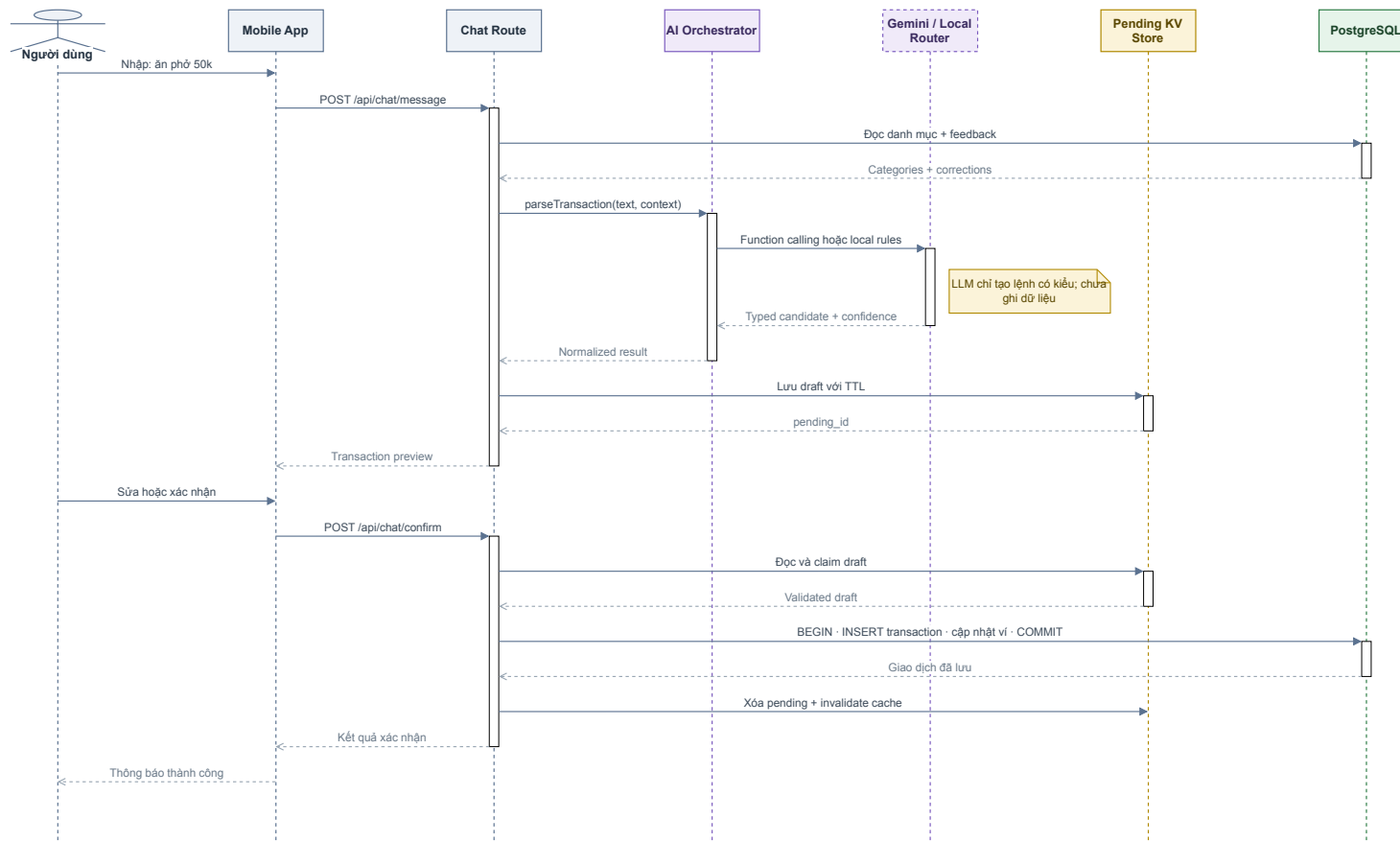
Figure 21: Sequence diagram for text transaction entry. The LLM sits outside the data-writing transaction.
