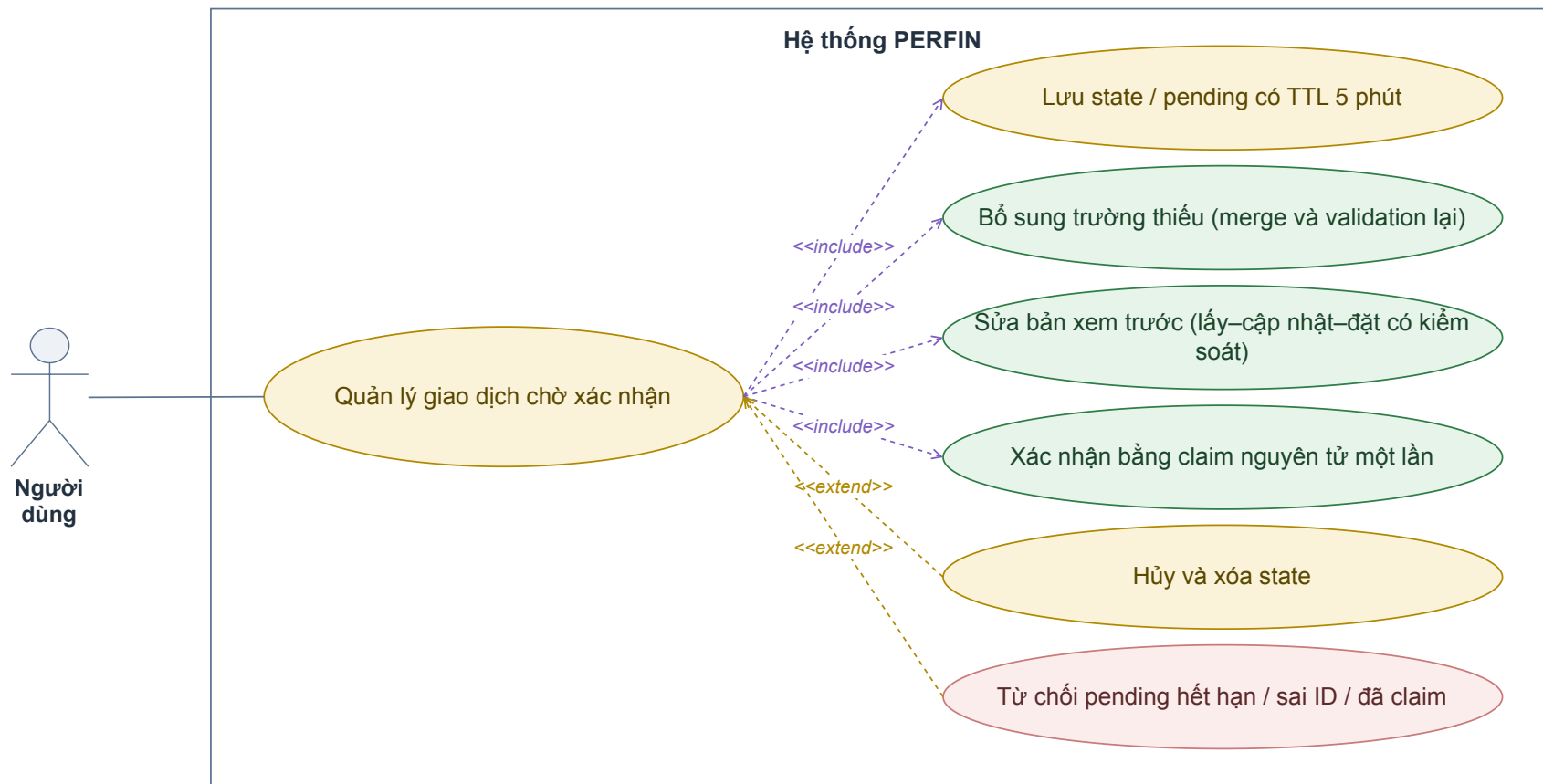
Figure 5: Detailed use case for FR-03 — clarification and pending transactions.
