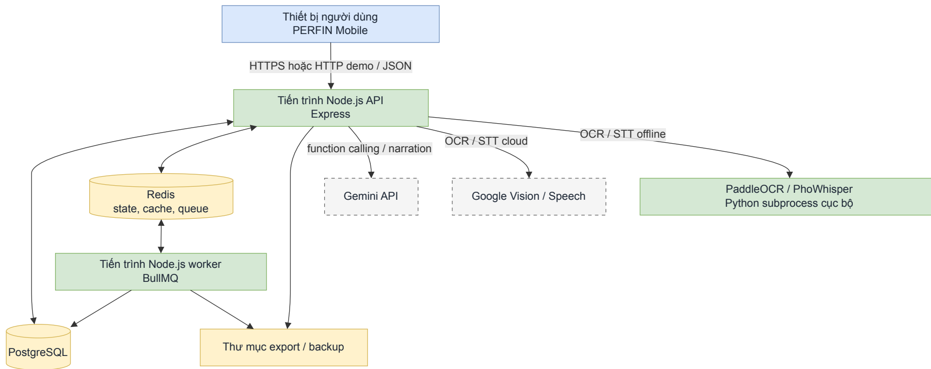
Figure 3: Prototype deployment diagram. The frontend, API, worker, PostgreSQL and Redis belong to the demo environment; the AI provider is called over the network.
