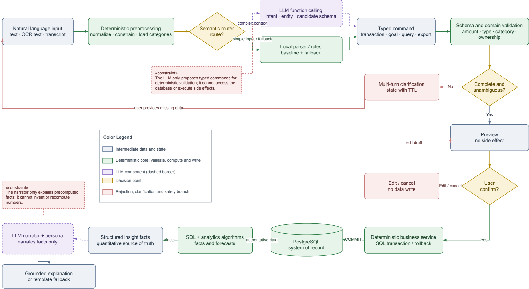
Figure 3.7: LLM responsibility boundary: typed drafts and narration remain outside validation, calculation and data-write authority.
