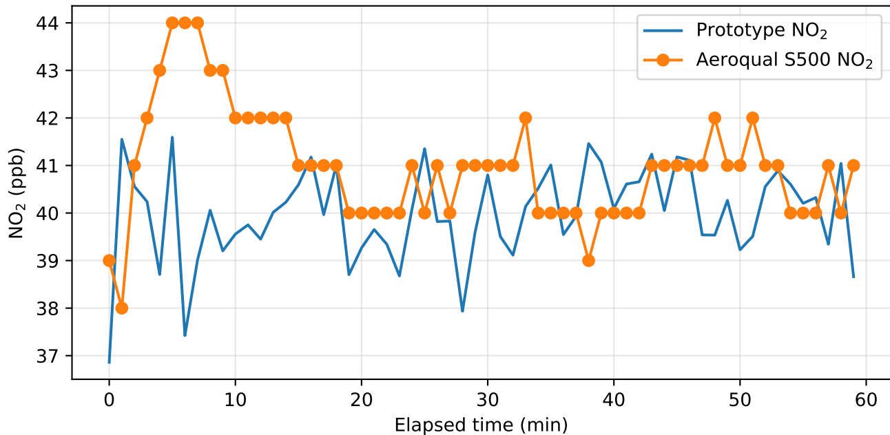
NO 2 one-hour co-location comparison
